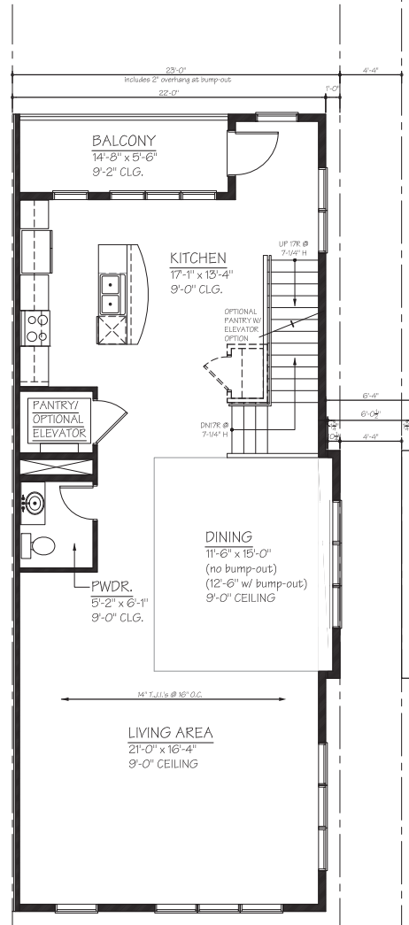
Main Living Level - 1,165 square feet
