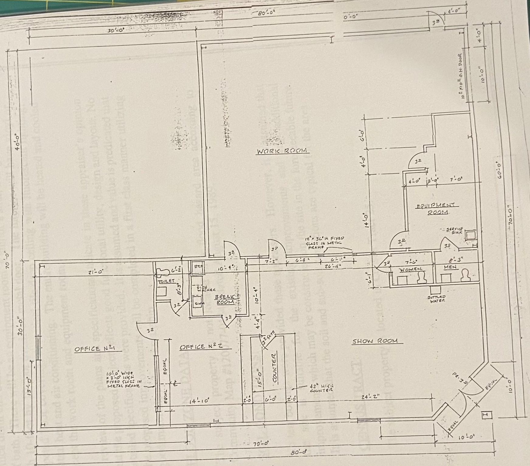
FLOOR PLAN
