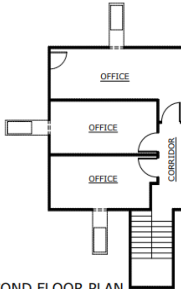
SECOND FLOOR PLAN EXISTING 1/4" = 1'-0"
