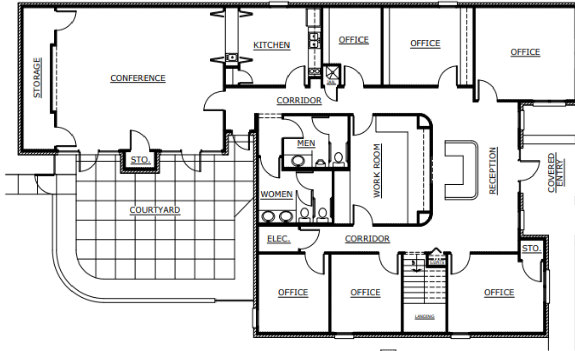
FIRST FLOOR PLAN EXISTING 1/4" = 1'-0"
