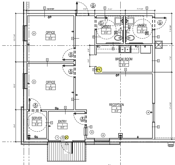
OFFICE FLOOR PLAN | BUILDINGS 4, 8 AND 9
