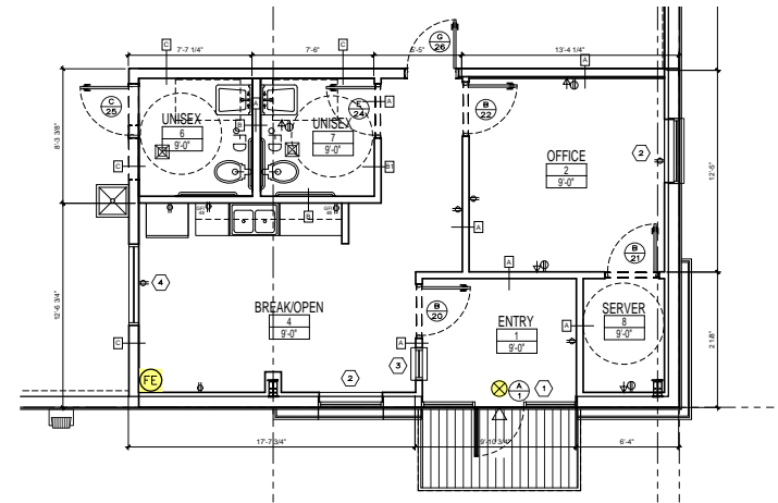
OFFICE FLOOR PLAN | BUILDINGS 6 AND 7
