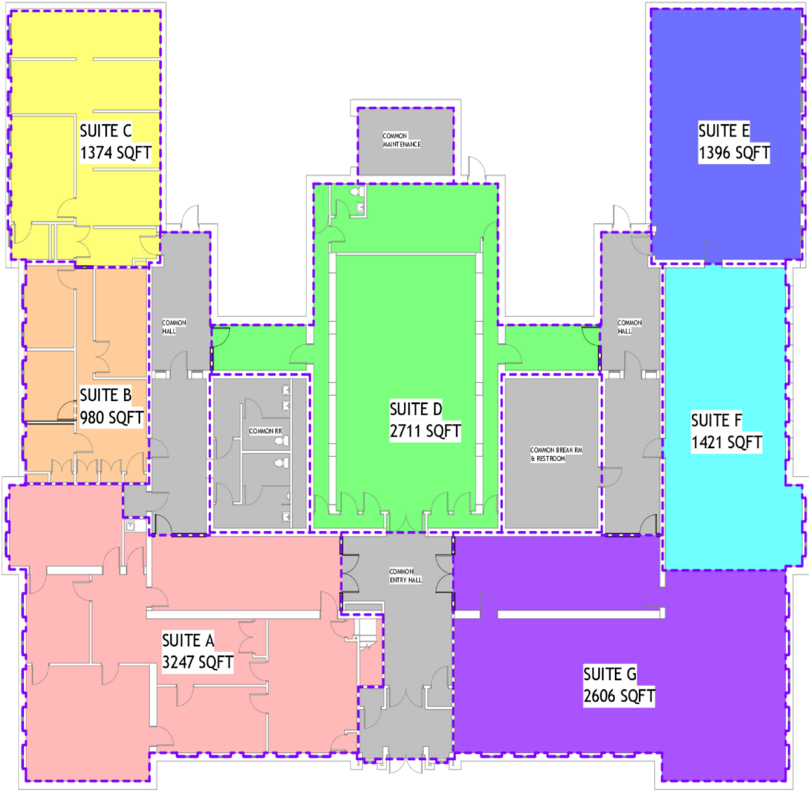
① RENTABLE FLOOR PLAN 1/8" = 1'-0"
