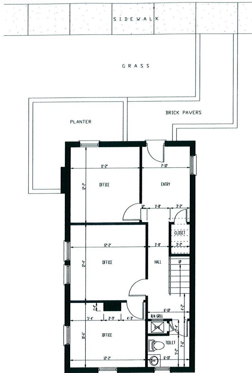
444 FIRST FLOOR PLAN
