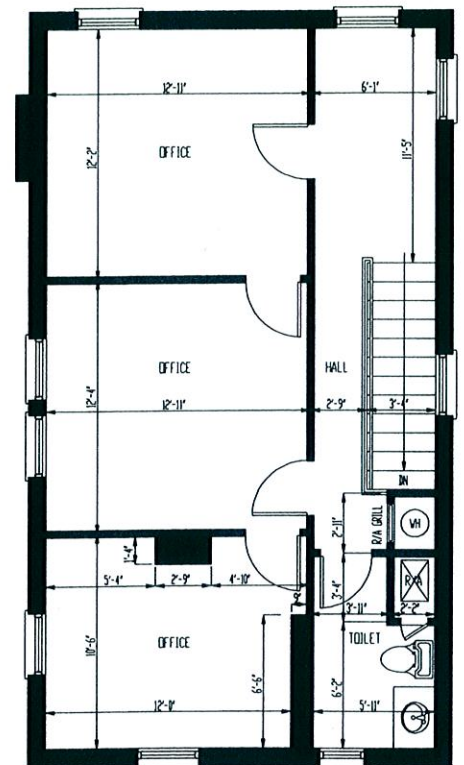
444 SECOND FLOOR PLAN
