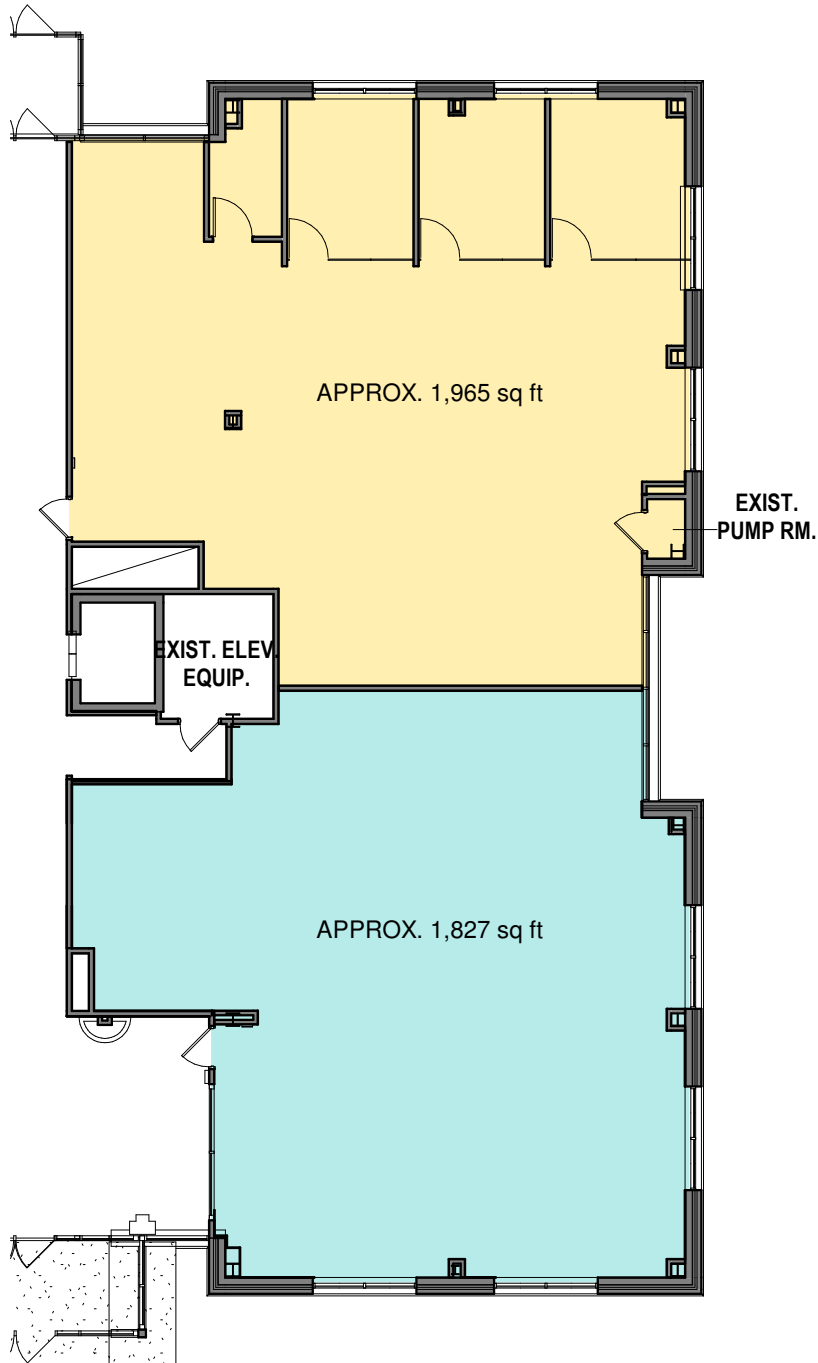
① PARTIAL FIRST FLOOR PLAN - EAST 3/32" = 1'-0"
