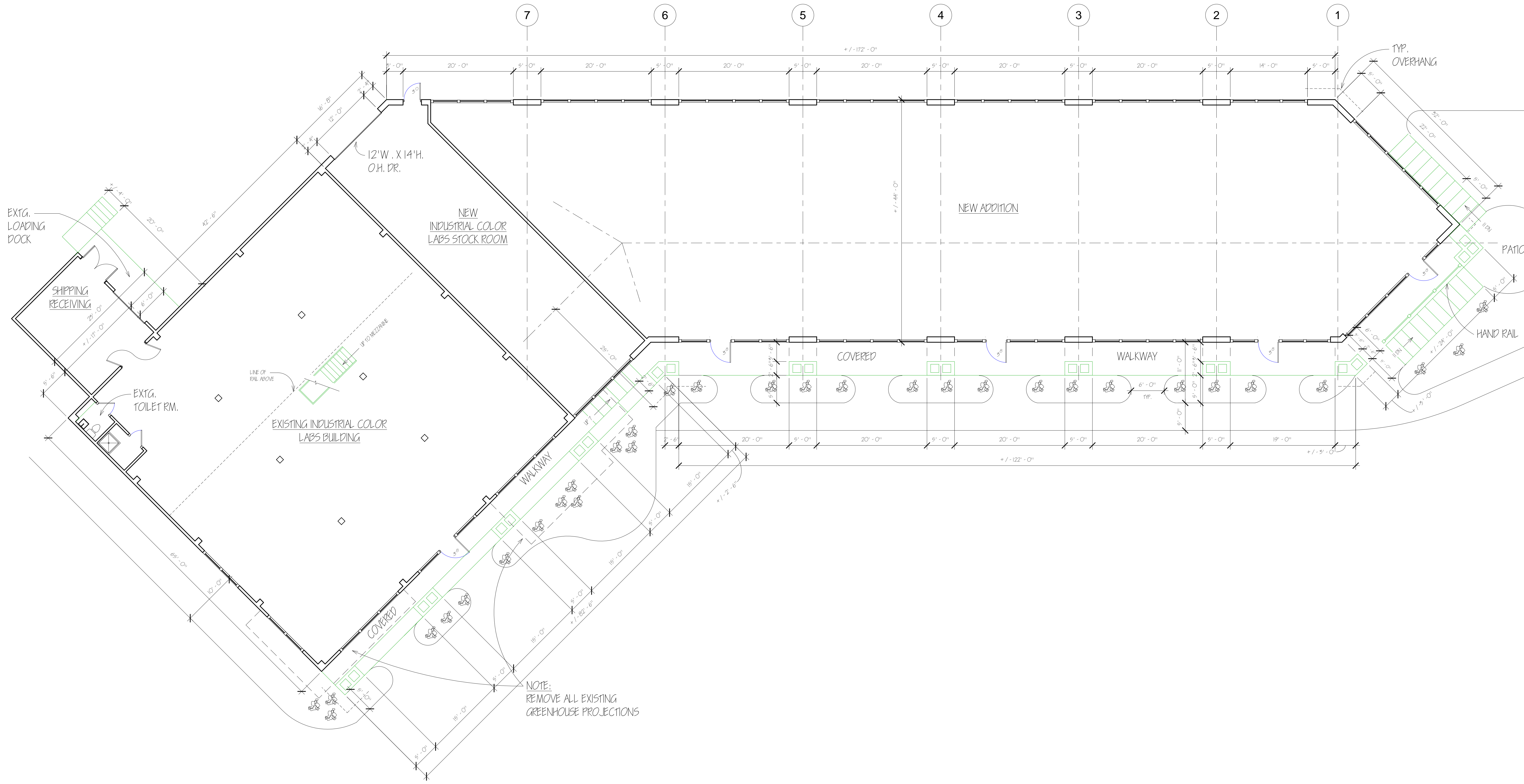
1 MAIN LEVEL PLAN 1/8" = 1'-0"
