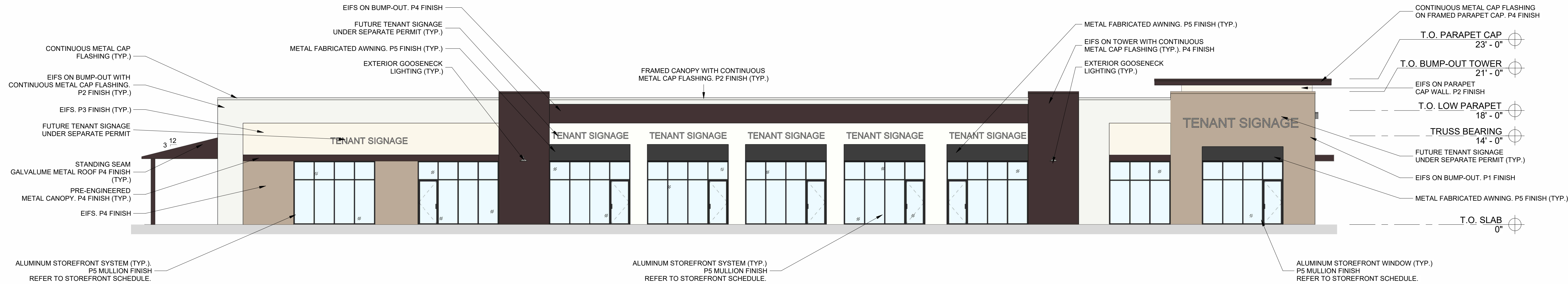
2 A2.0 SOUTH ELEVATION 1/8" = 1'-0"
