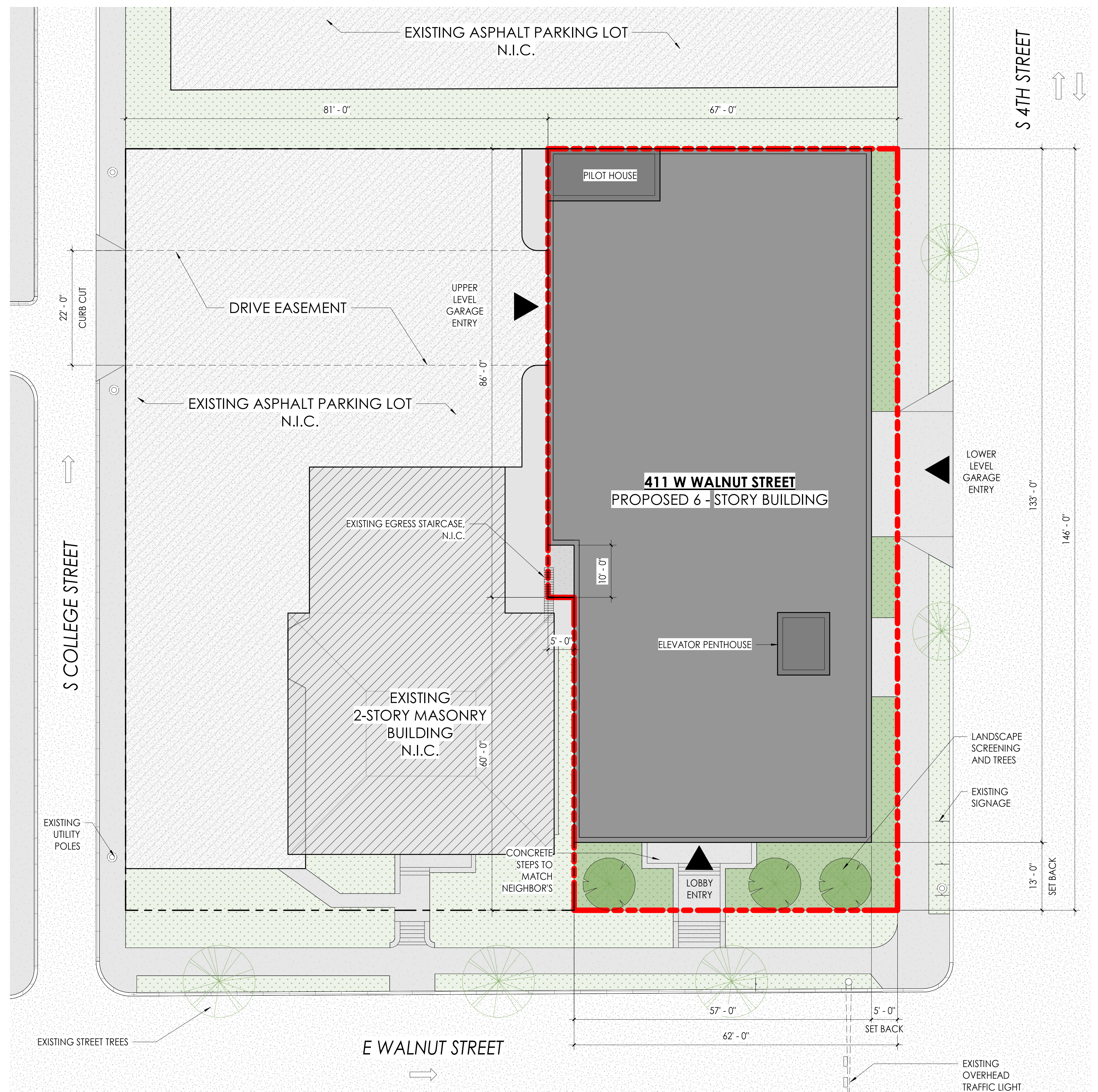
1 | SITE PLAN
