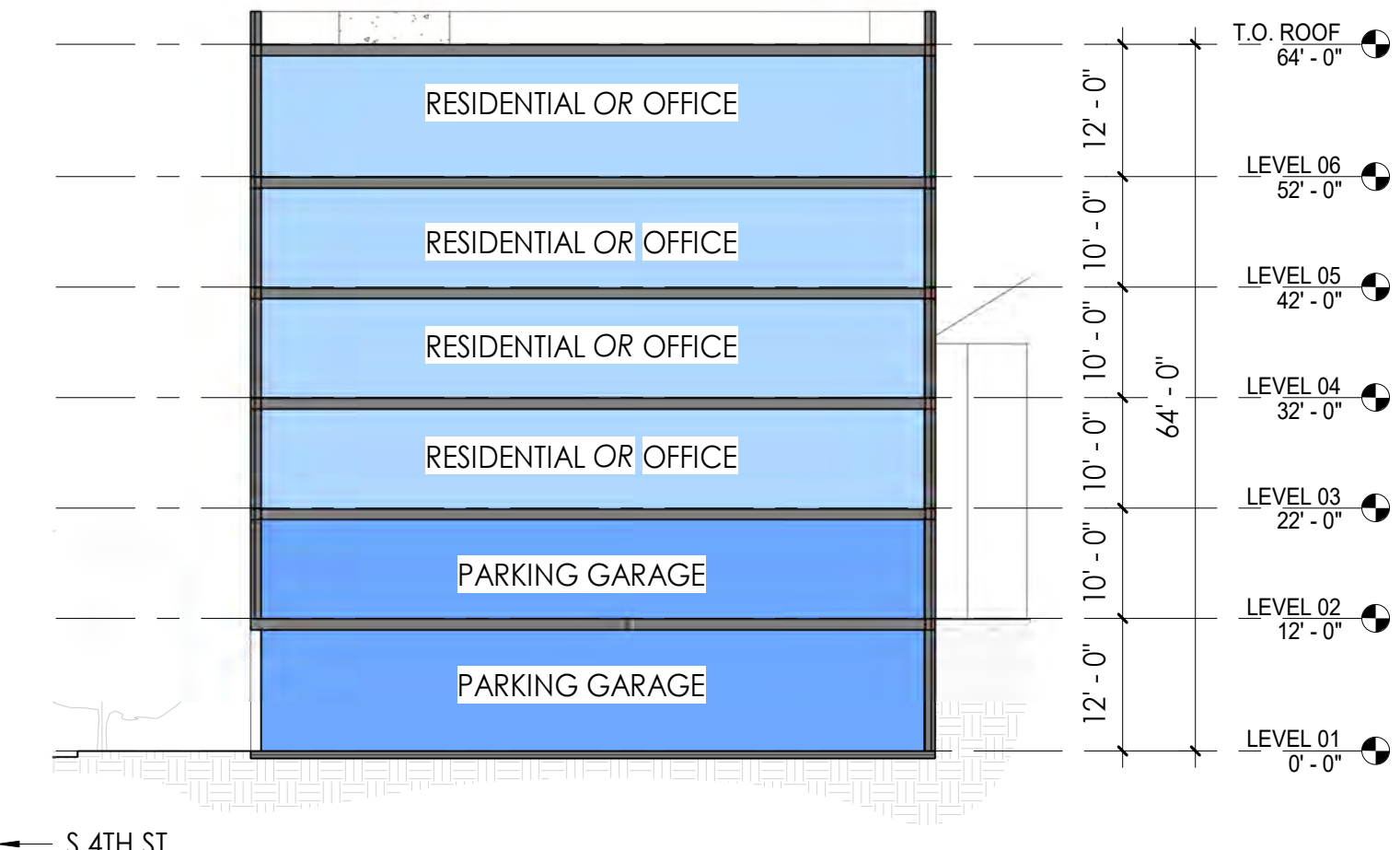
3 | DIAGRAMATIC CROSS SECTION
