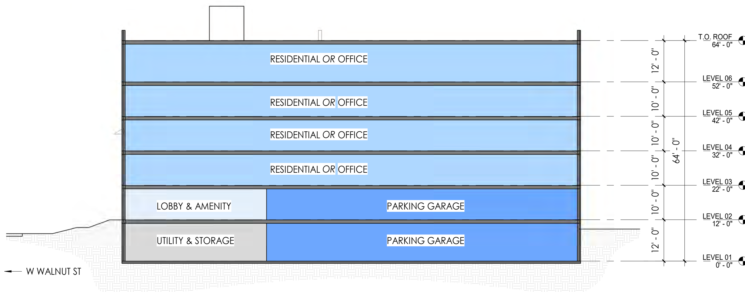
2 | DIAGRAMATIC LONGITUDINAL SECTION
