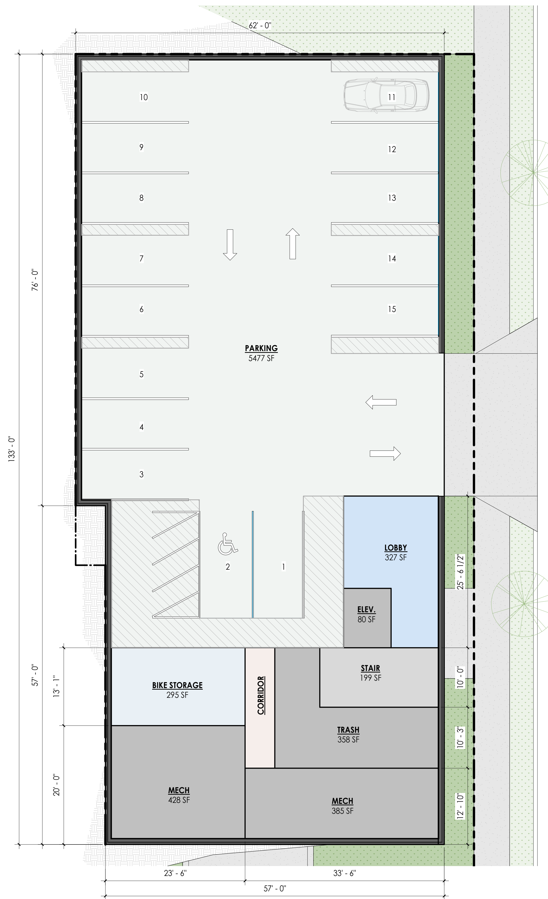
1 | LEVEL 01 FLOOR PLAN
