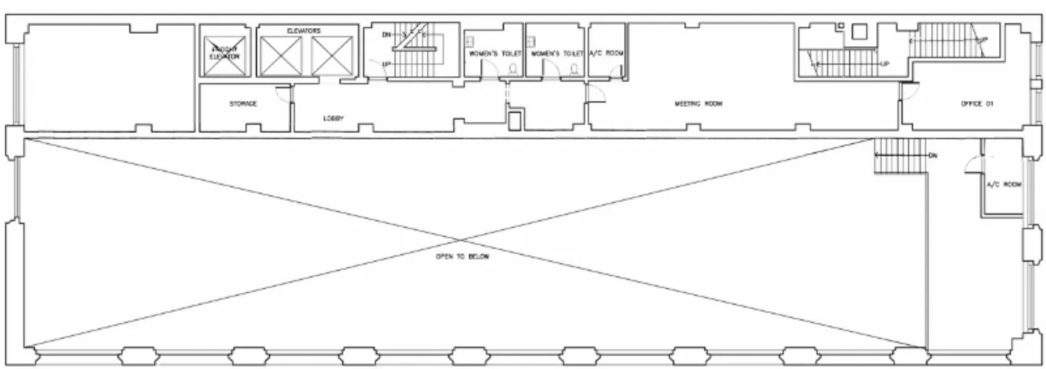
MEZZANINE FLOOR PLAN
