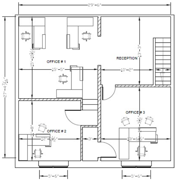
EXISTING 2ND FLOOR SCALE: 1/4" = 1'-0"
