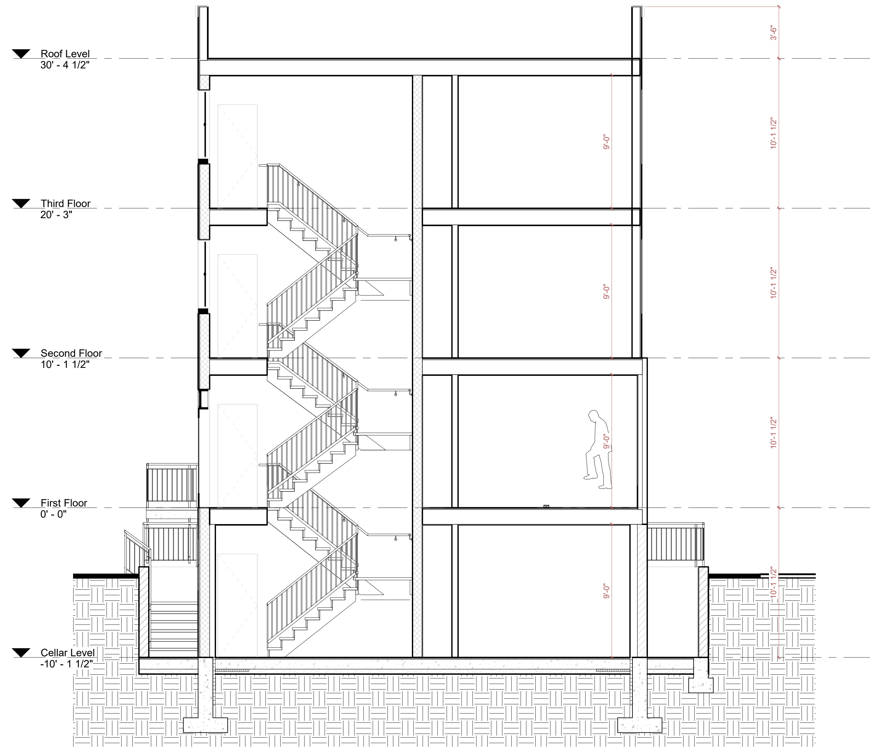
1 Section 1 1/4" = 1'-0"
