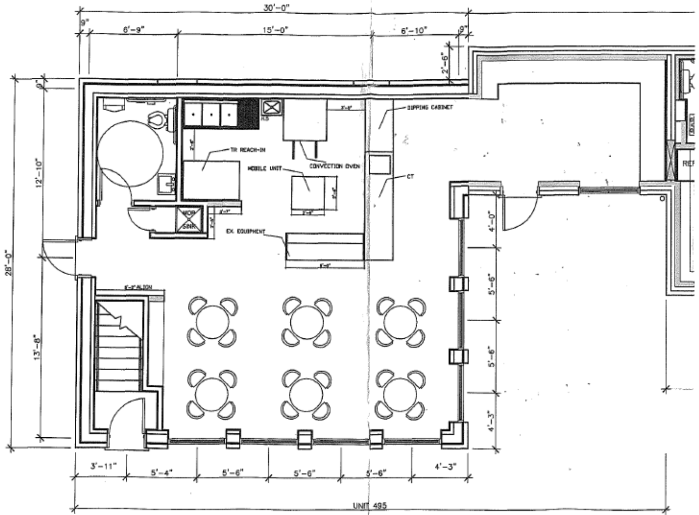
FIRST FLOOR PLAN SCALE: 3/16" = 1'-0"
