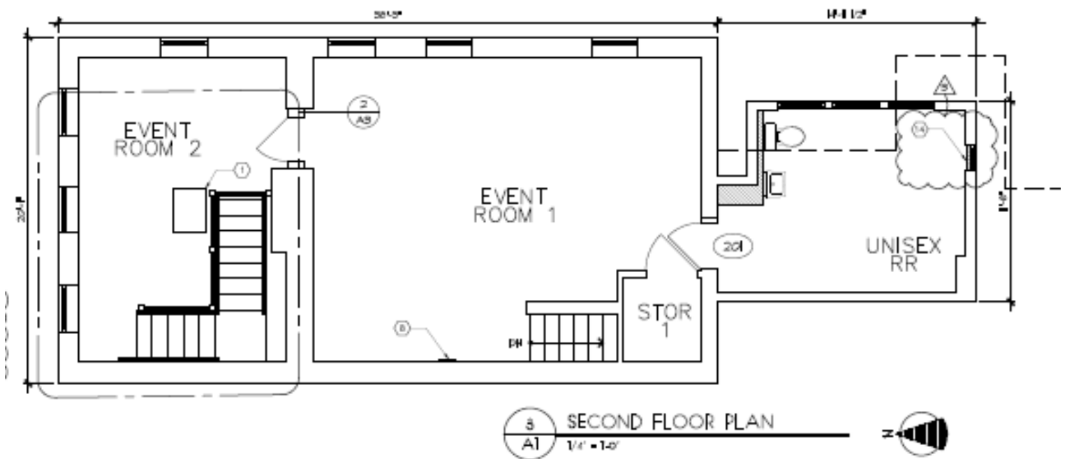
Second Level Floor Plan
