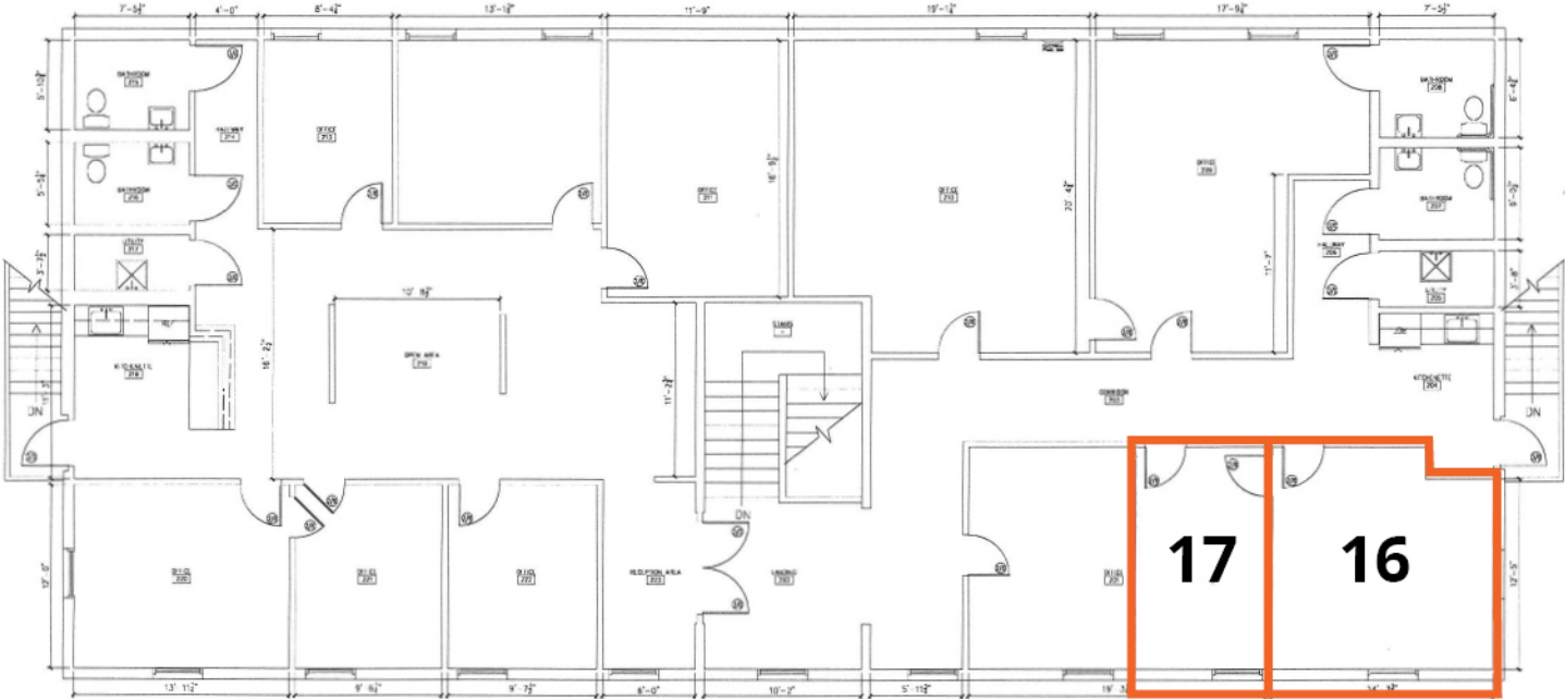
EXISTING SECOND FLOOR PLAN 3618 ASHLEY PHOSPHATE RD N CHARLESTON, SC 29418 SCALE: 1/4" = 1'-0" 3,948 SQUARE FOOT 12/05/2022
