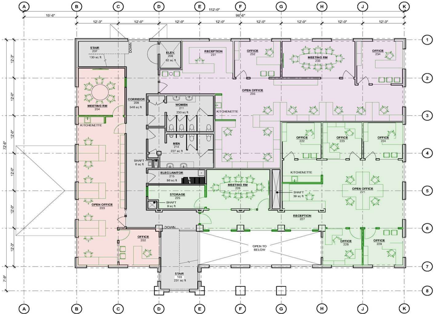
SECOND FLOOR PLAN - NEW CONSTRUCTION
