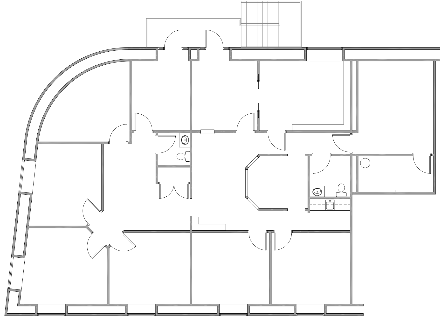
1 SECOND FLOOR (SUITE 300/400) 2,961 SQ FT SCALE: 1/8" = 1'-0"
