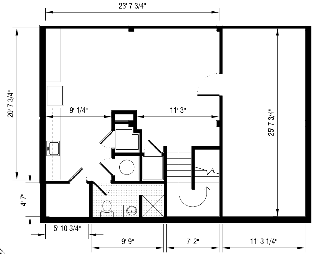
01 2nd Floor Plan
