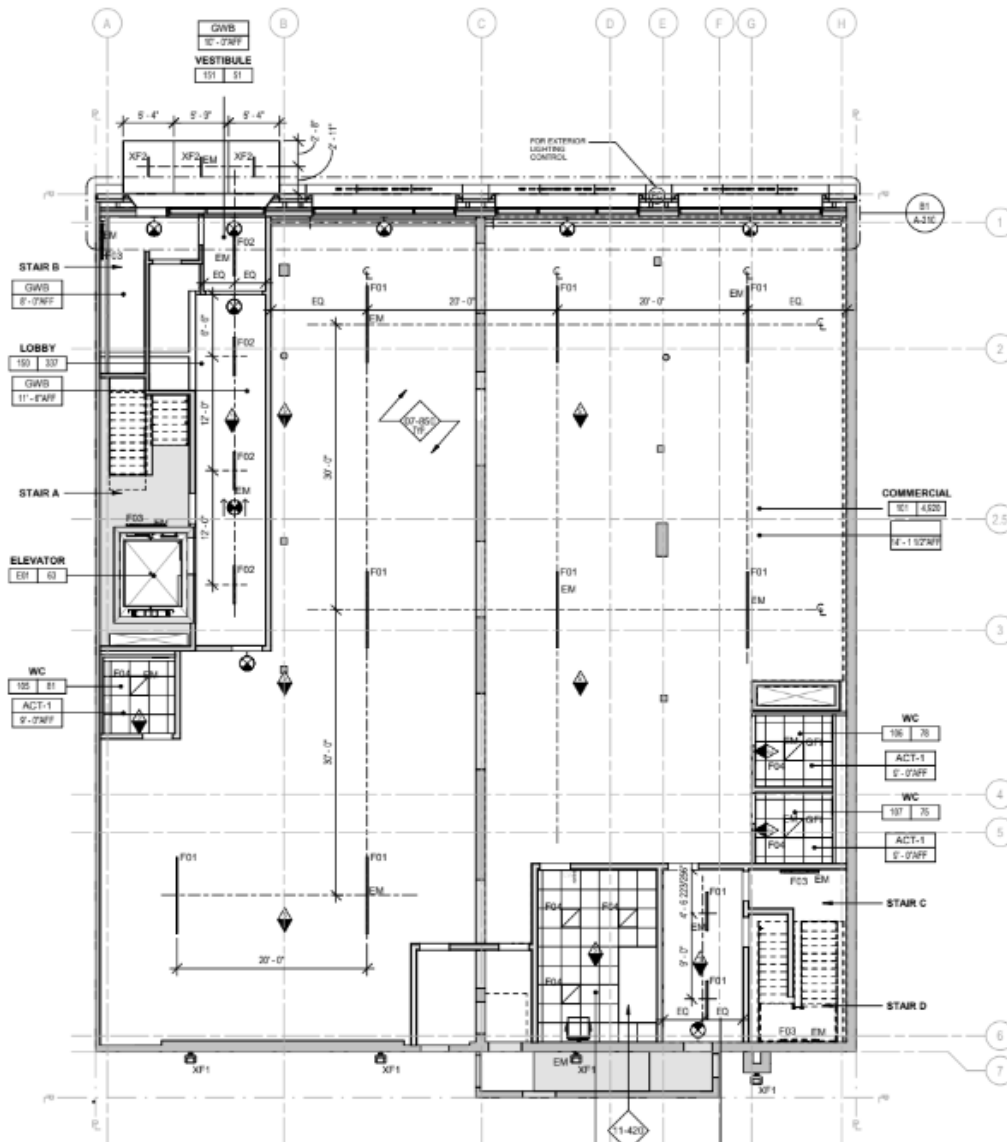
Ground Floor
