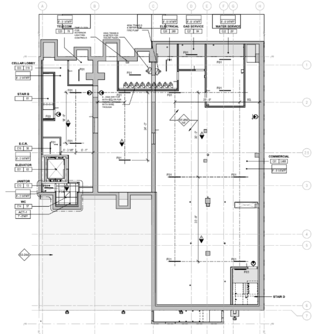
Cellar Level
