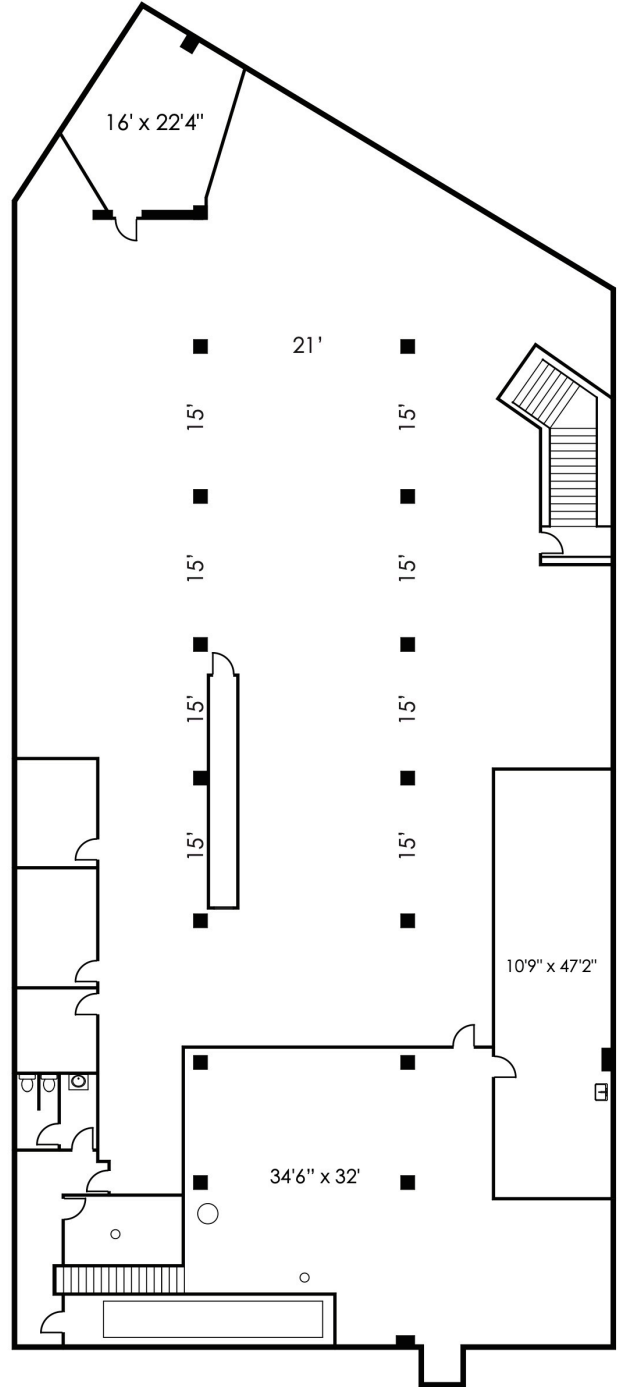
BASEMENT Ceiling Height: 11'
