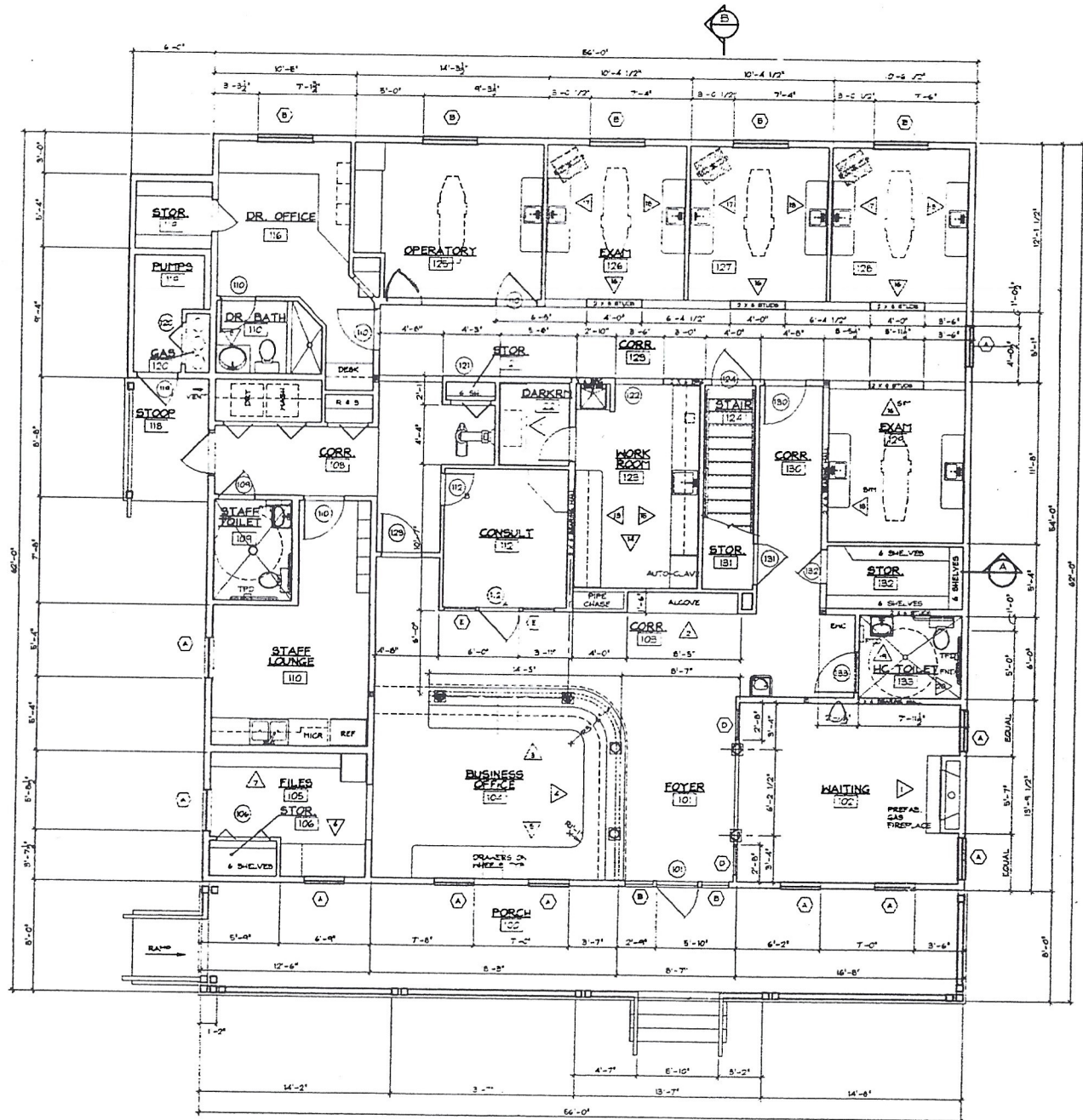
FLOOR PLAN 1/4" = 1'-0" 2,400.0 SF
