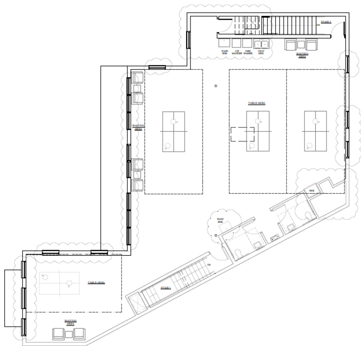
2 SECOND FLOOR PLAN SCALE: 1/8" = 1'-0"
