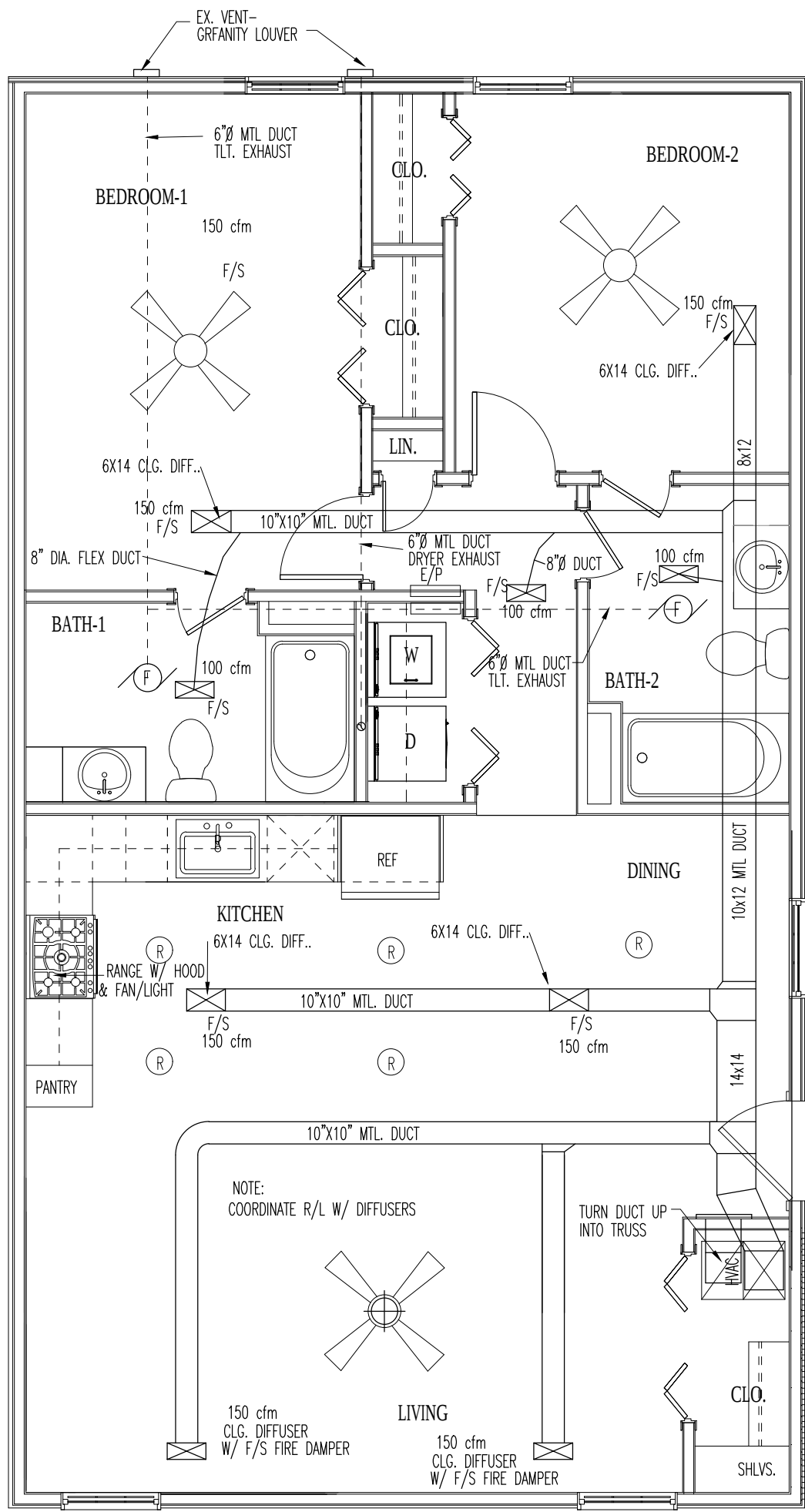
1 MECH. PLAN-B SCALE: 1/4"=1'-0"
