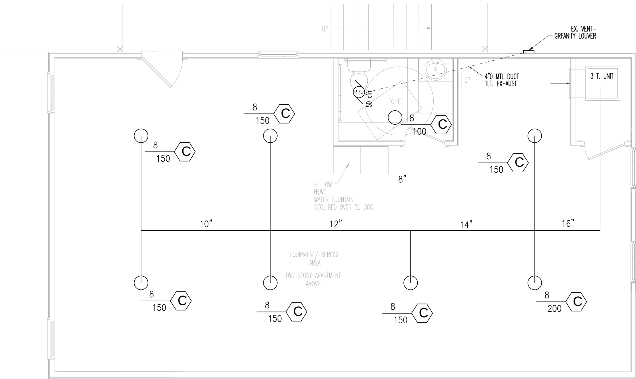
1 MECHANICAL PLAN SCALE: 1/4"=1'-0"
