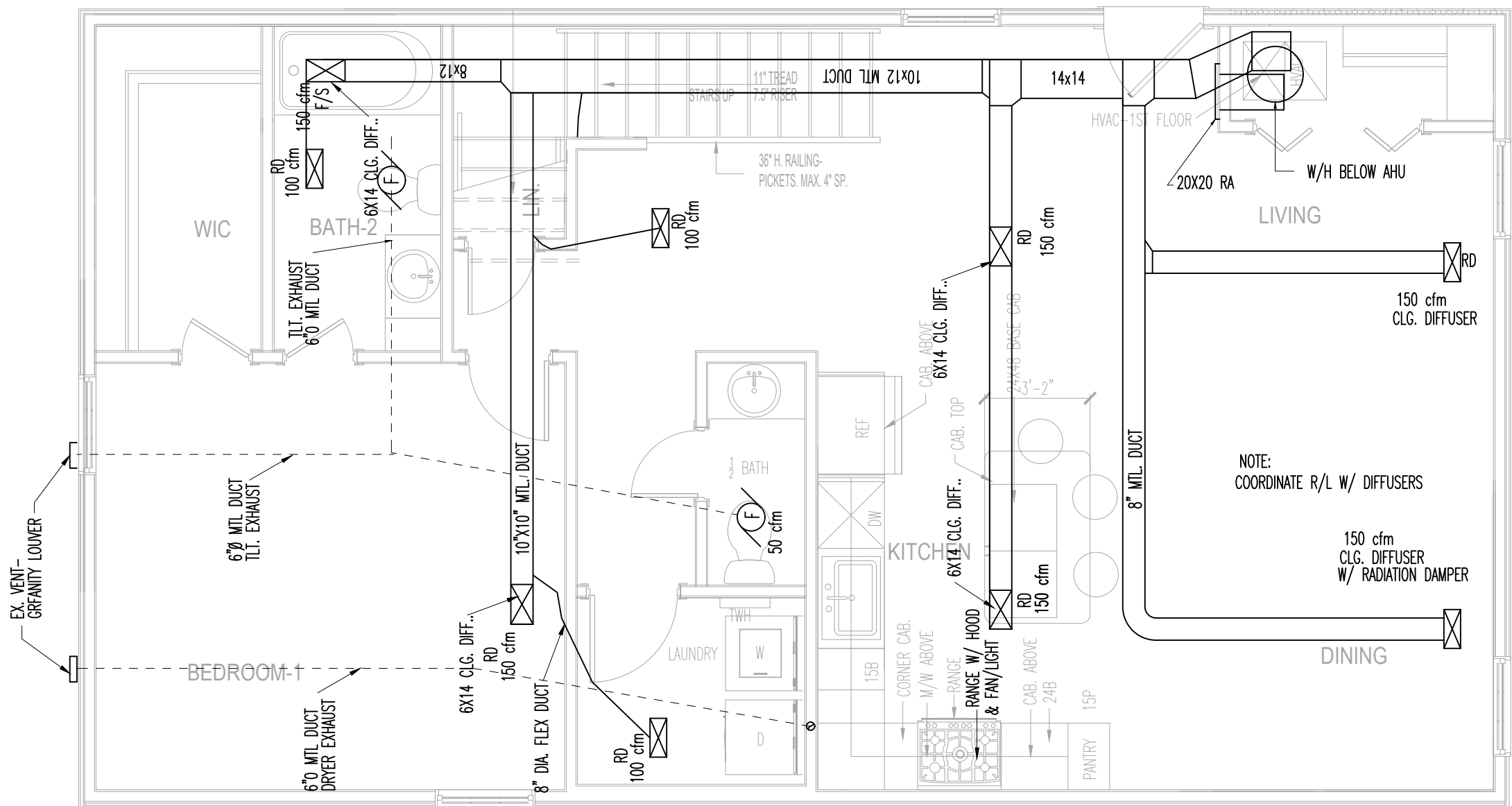
2 MECHANICAL PLAN-2ND FLOOR SCALE: 1/4"=1'-0"
