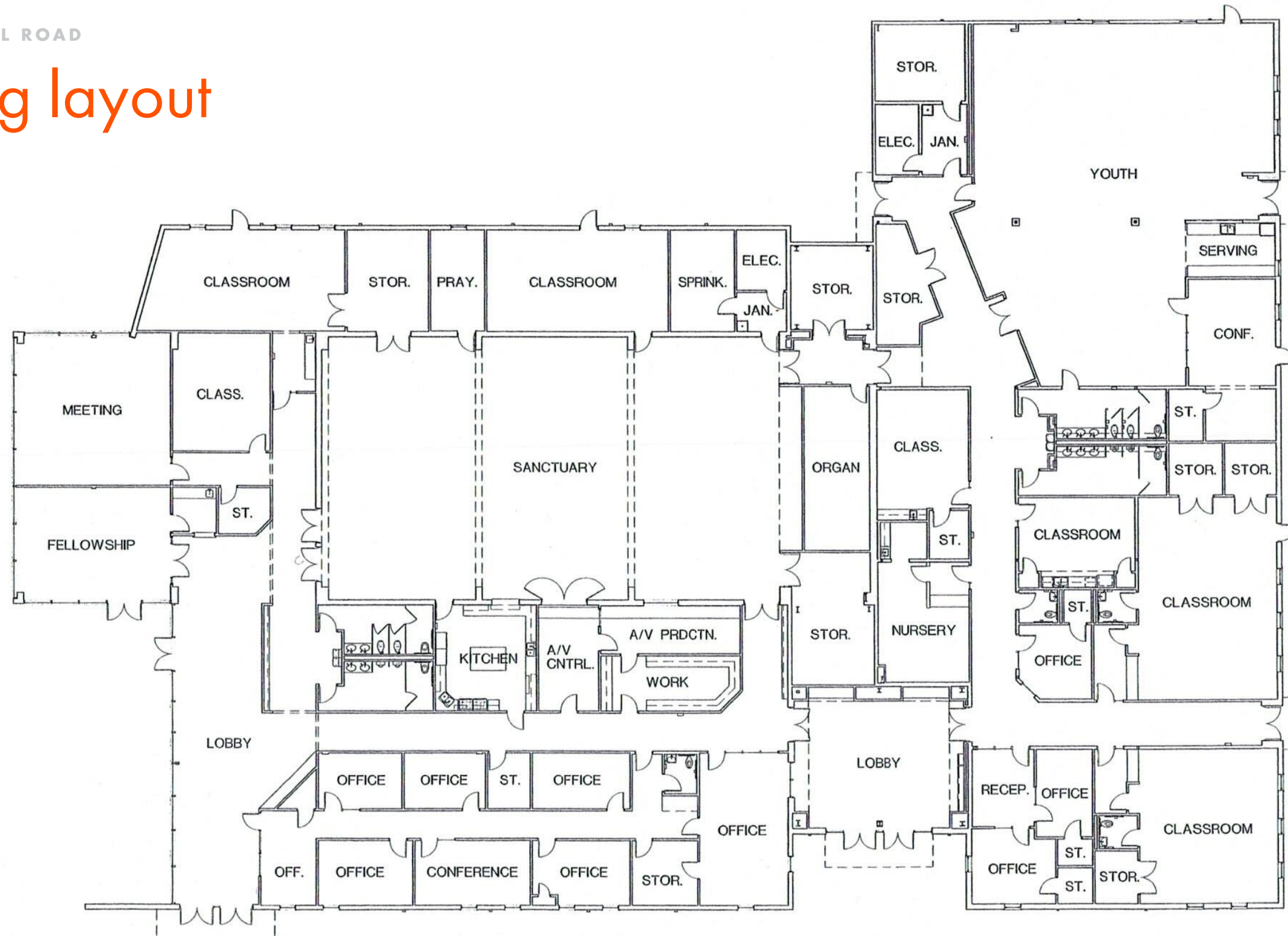
1" = 20'-0" FLOOR PLAN
