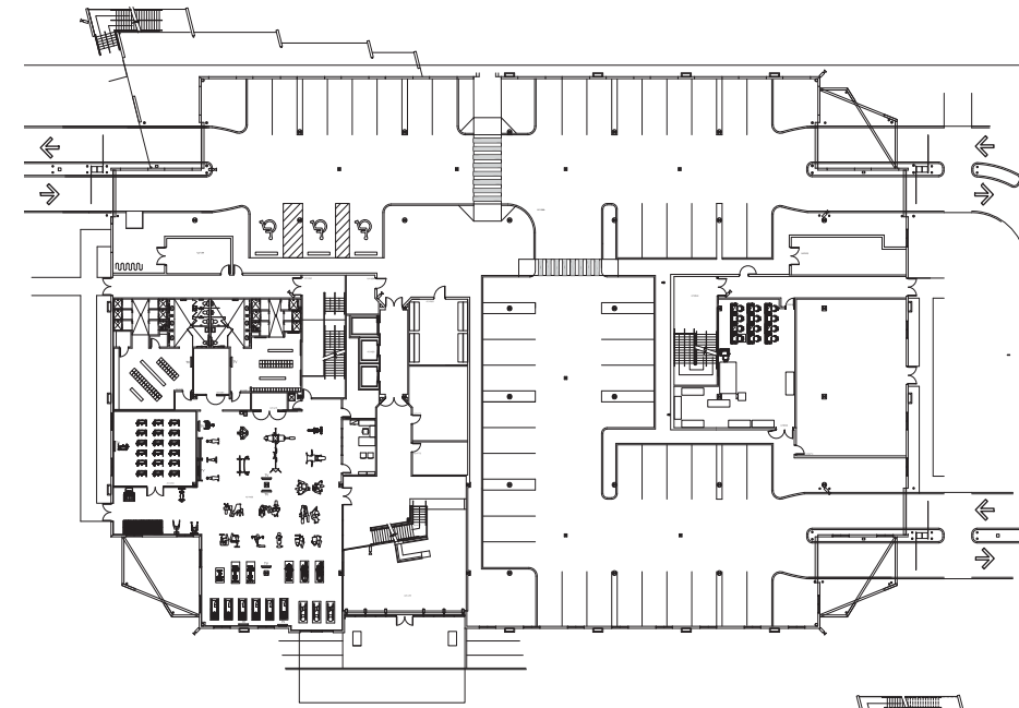
Floor 1 20,755 RSF
