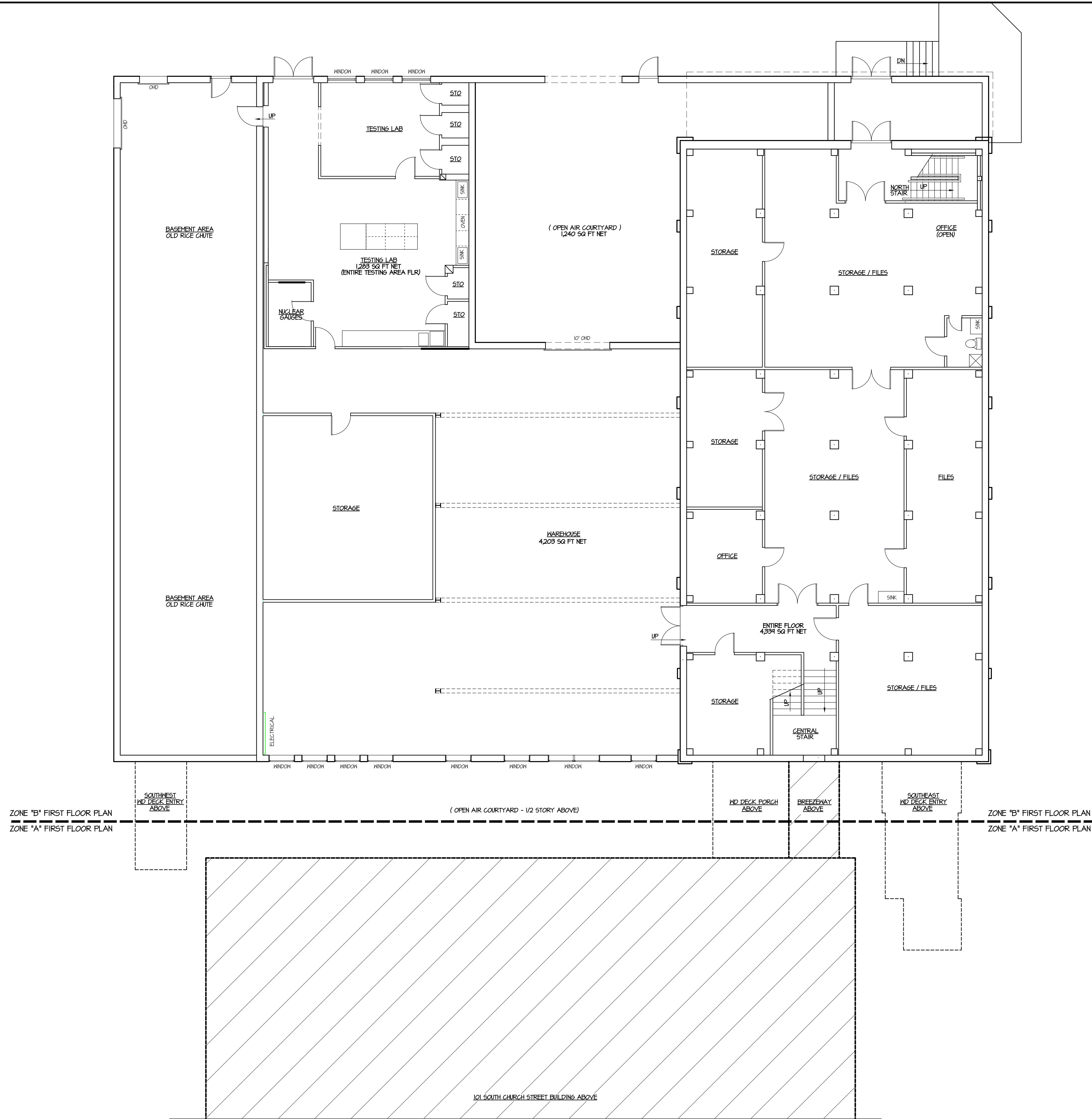
FIRST FLOOR PLAN - ZONE A & B 1/8"
