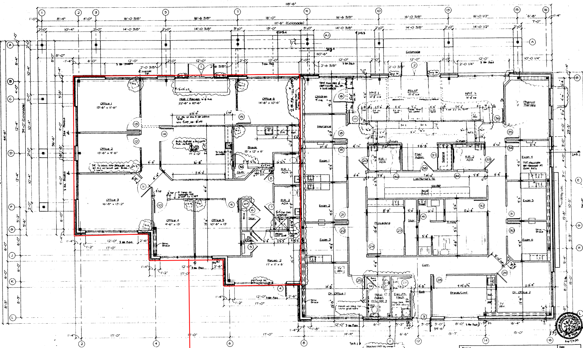
Floor Plan Scale: 1/4" = 1'-0" 5544 SF
