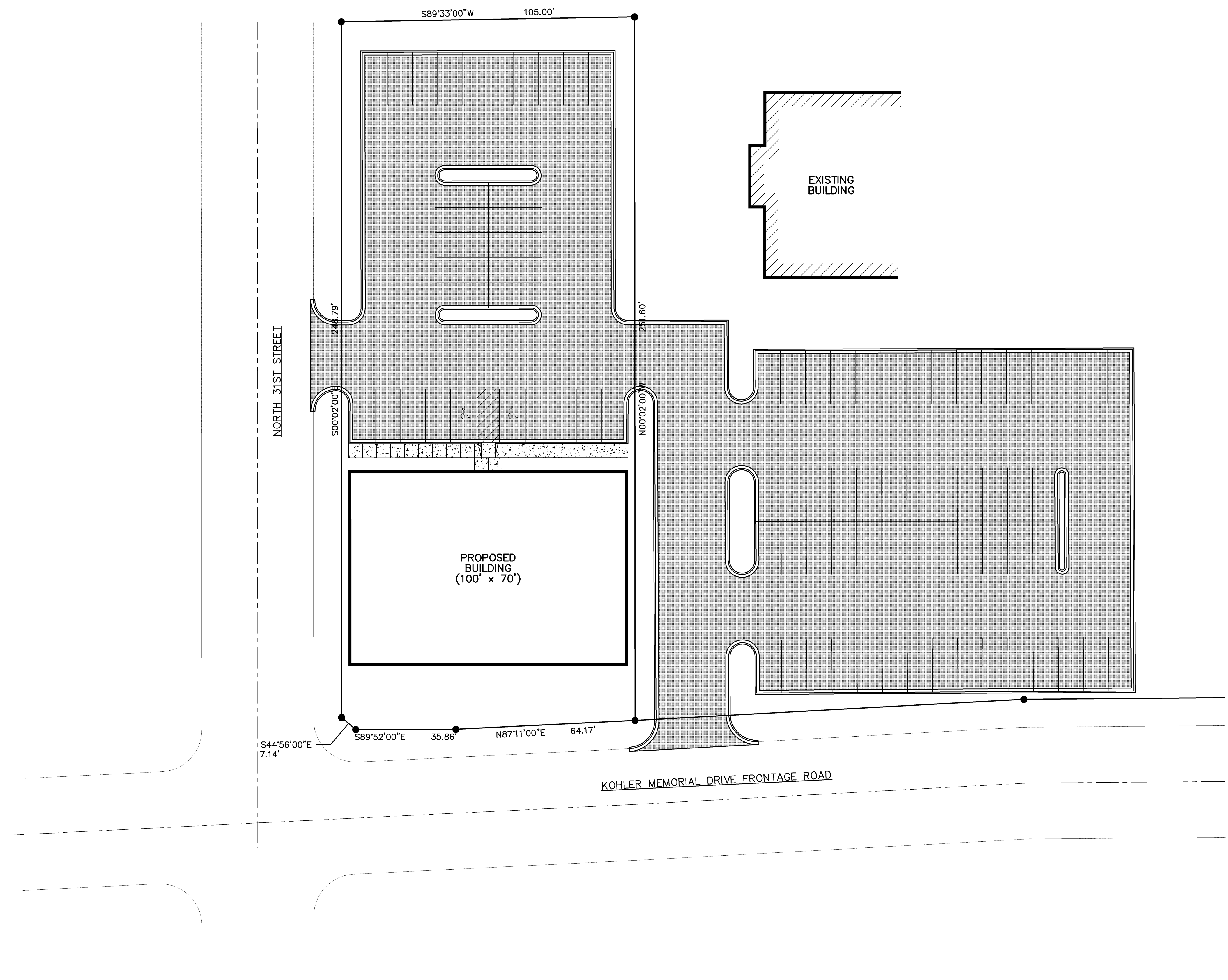
OPTION #1 - PROPOSED SITE PLAN SCALE: 1" = 20'-0"
