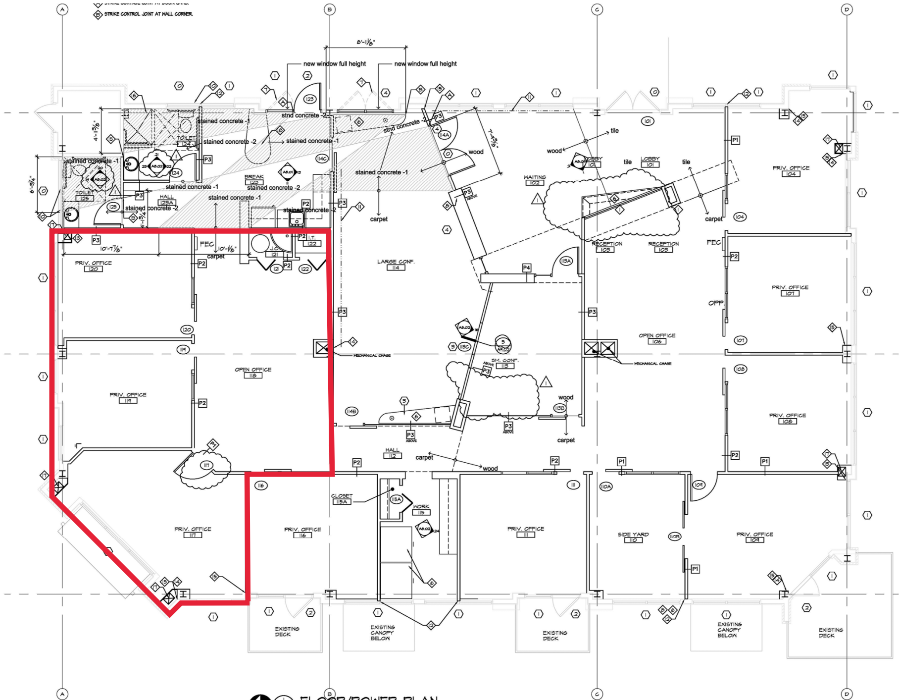
FLOOR/POWER PLAN SCALE: 1/4" = 1'-0"
