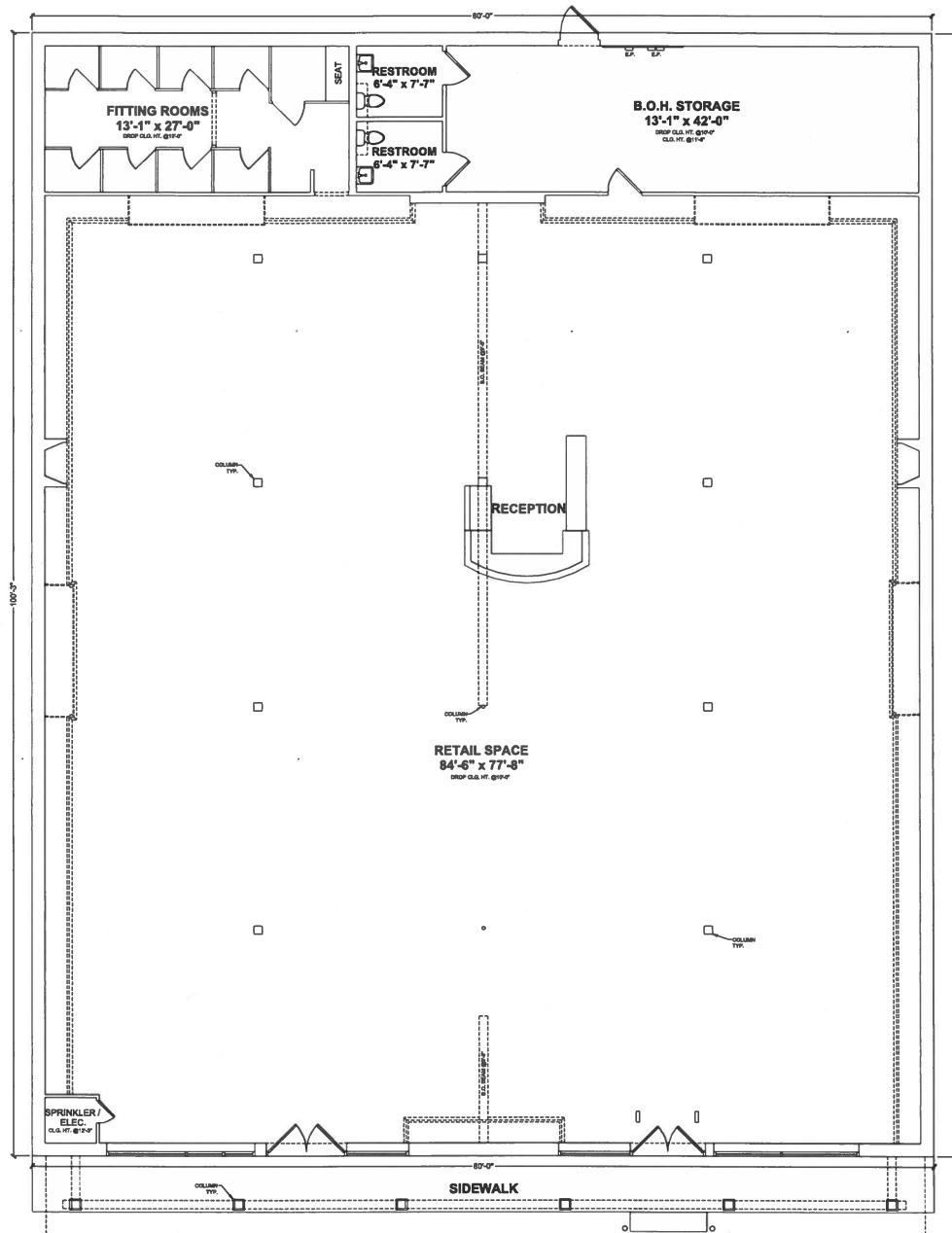
FIRST FLOOR PLAN Ceiling Height = See Drawing
