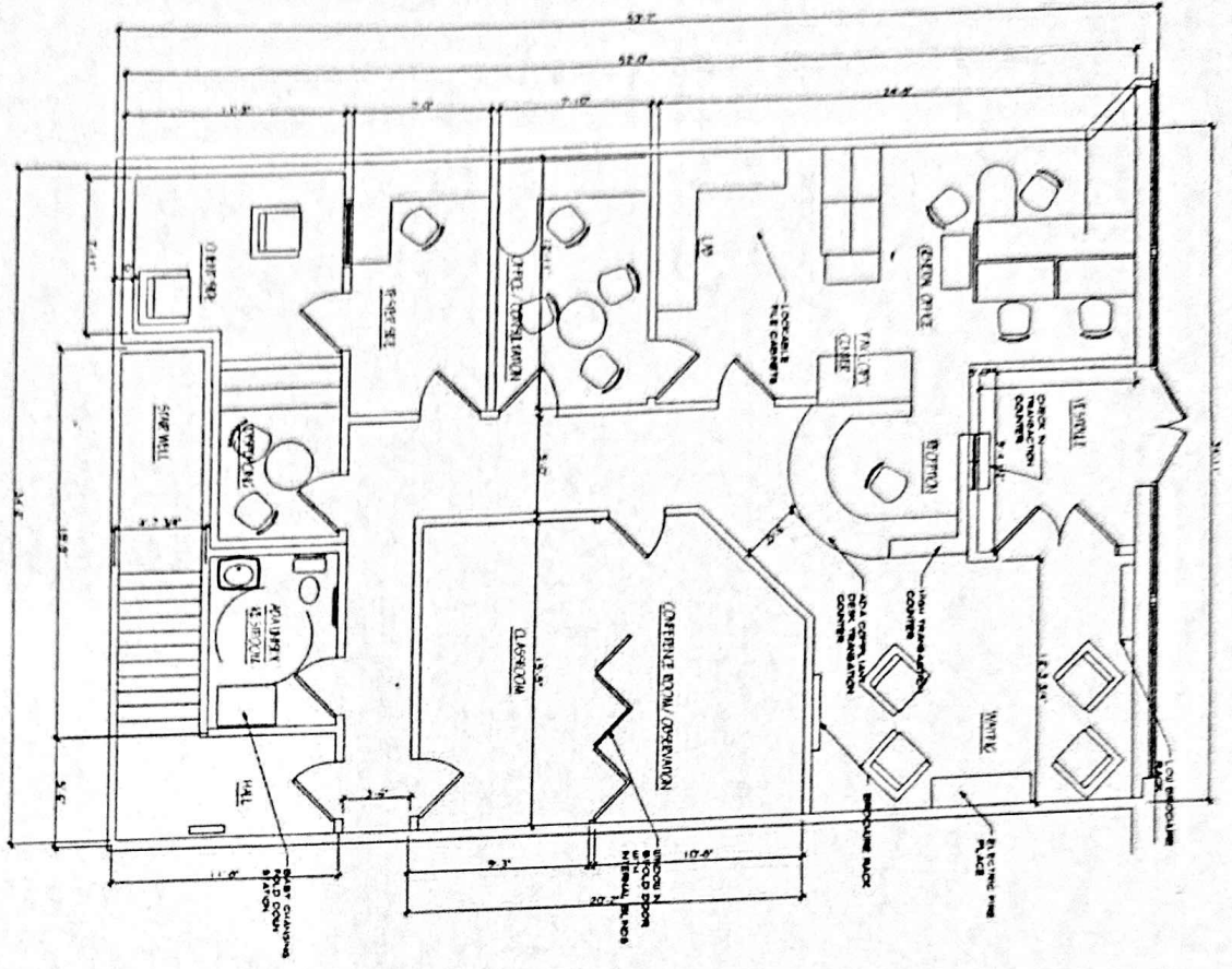
PROPOSED FLOOR PLAN SCALE: 1/8" = 1'-0"
