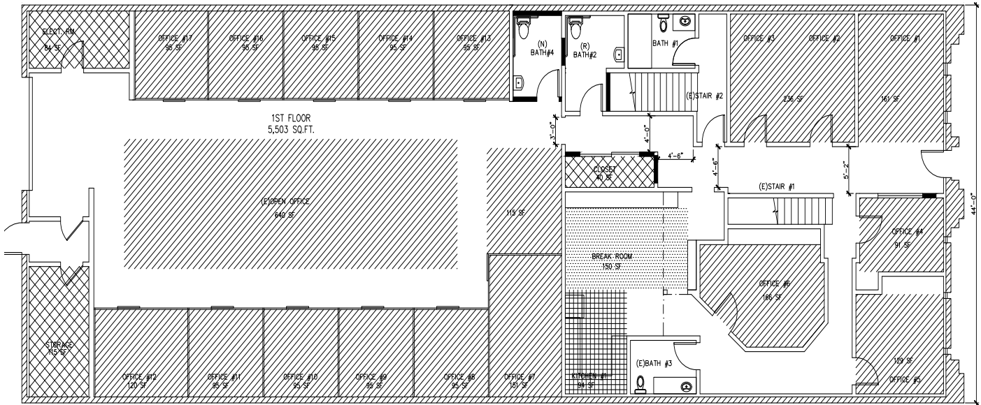
FIRST FLOOR PLAN 3/16"=1'-0"
