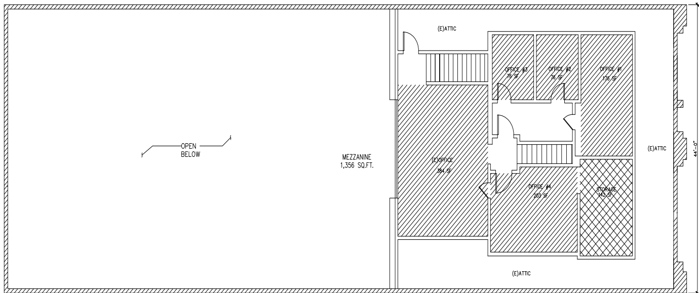
SECOND FLOOR PLAN 3/16"=1'-0"
