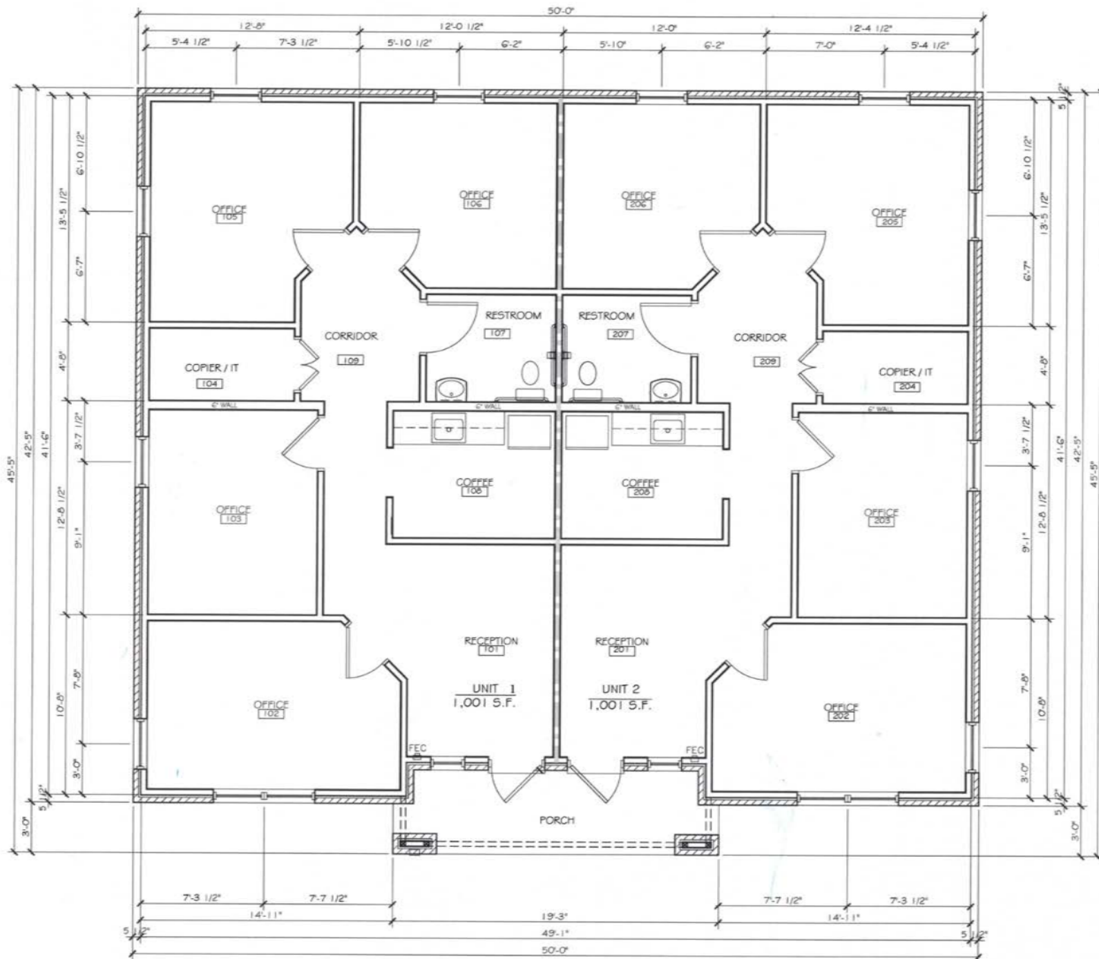
1 FLOOR PLAN 1/4" = 1'-0"
