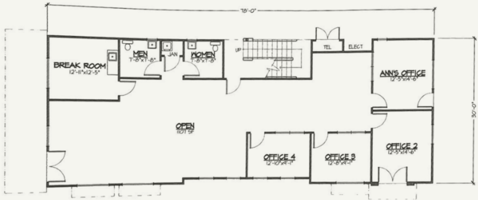
FIRST FLOOR PLAN 1/8" = 1'-0"
