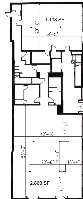
PEOPLES BANK 1ST FLOOR
