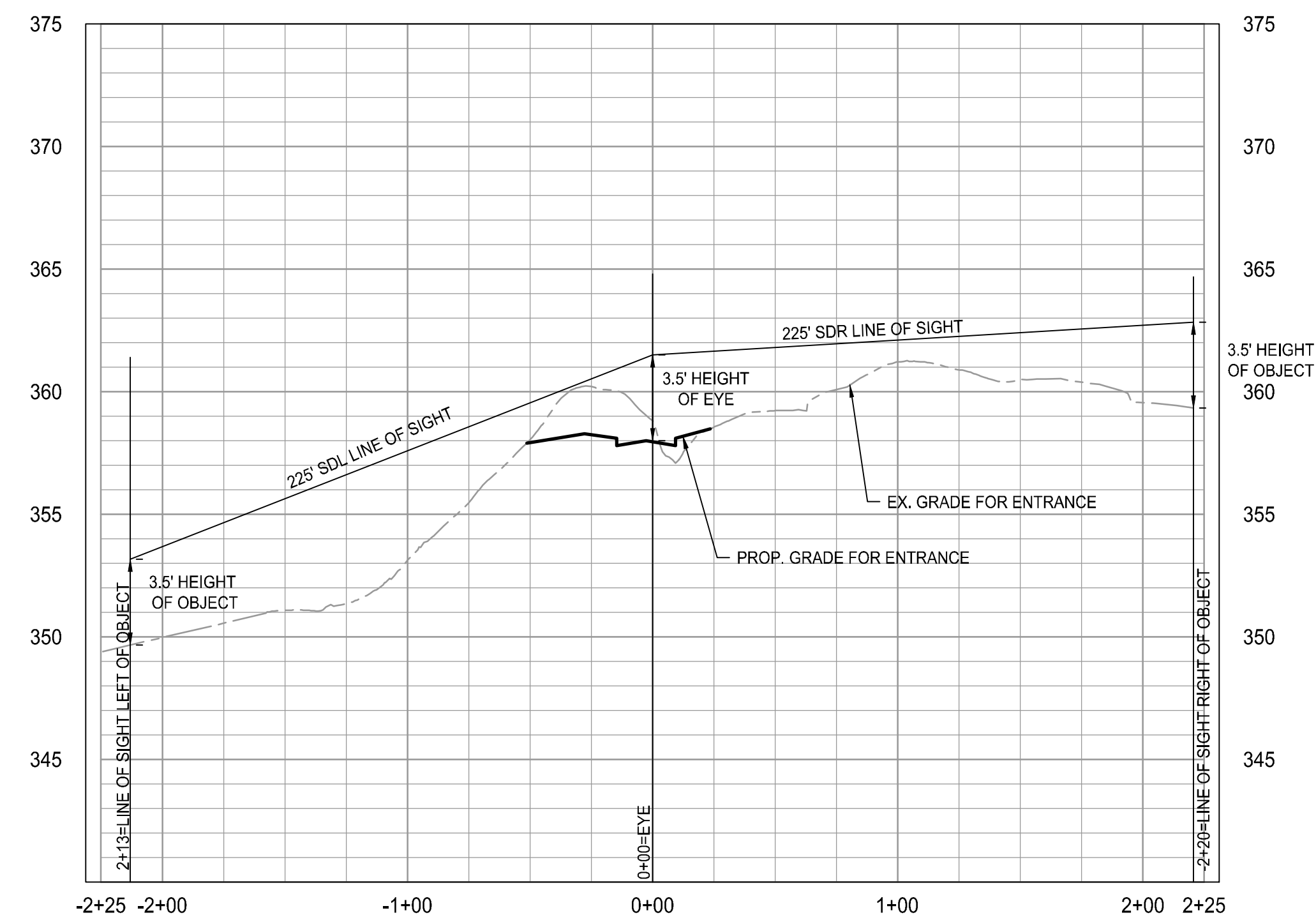
SIGHT DISTANCE OFFSITE PROFILE
