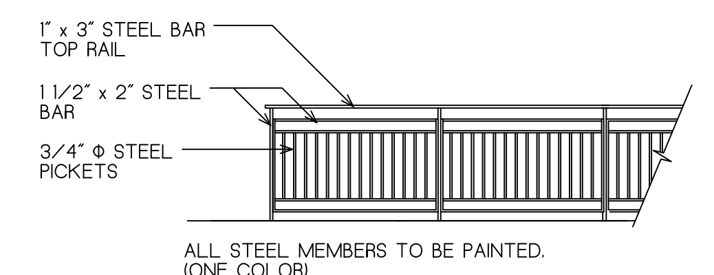
3 GUARD RAIL ELEVATION 1/4" = 1'-0"
