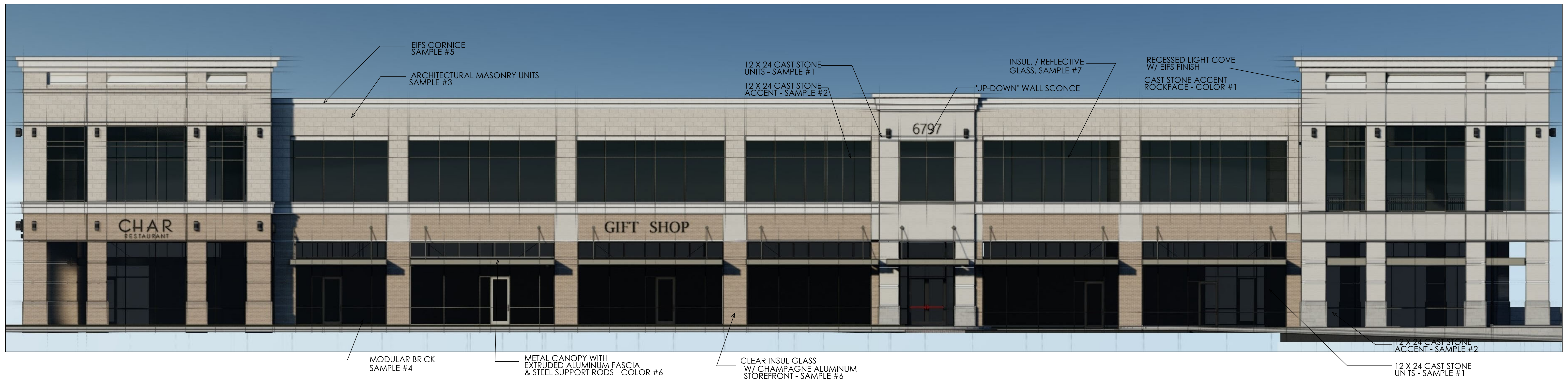
1 EAST ELEVATION 1/8" = 1'-0"
