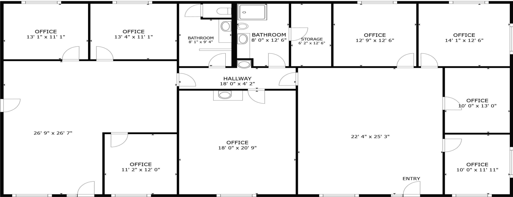
FLOOR PLAN
