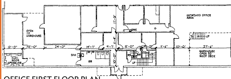
OFFICE FIRST FLOOR PLAN
