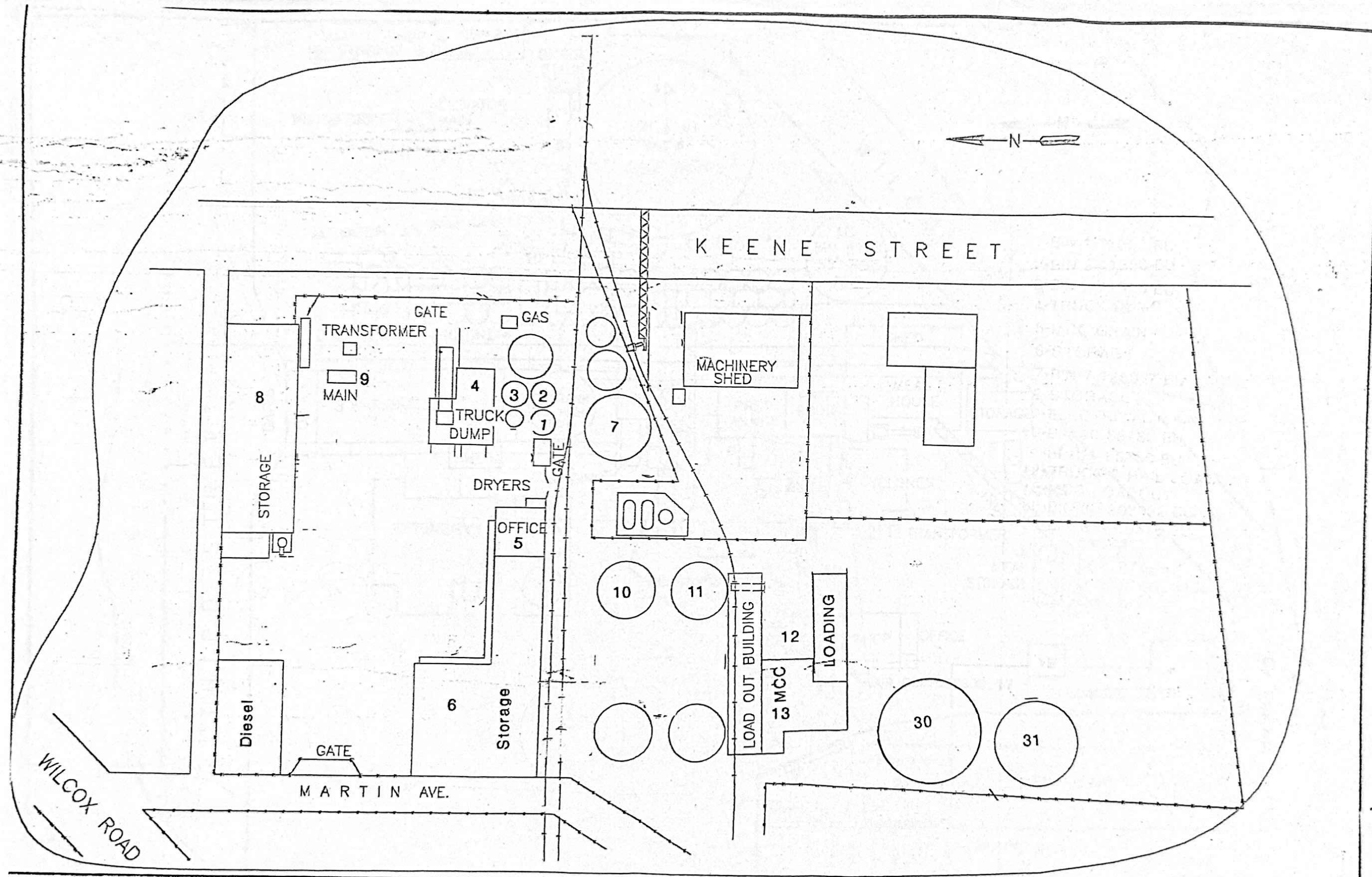
FIGURE 2-2B: SITE LAYOUT GRAIN OPERATIONS
