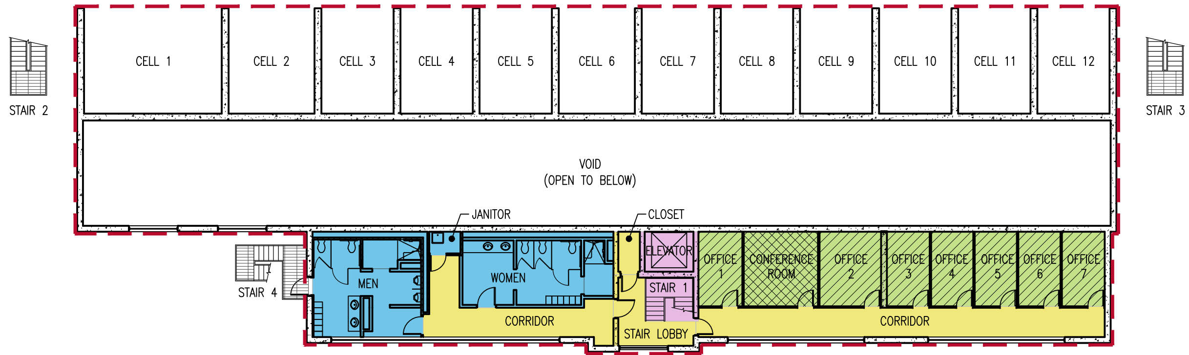
1 MEZZANINE FLOOR PLAN SCALE: 1/16" = 1'-0"
