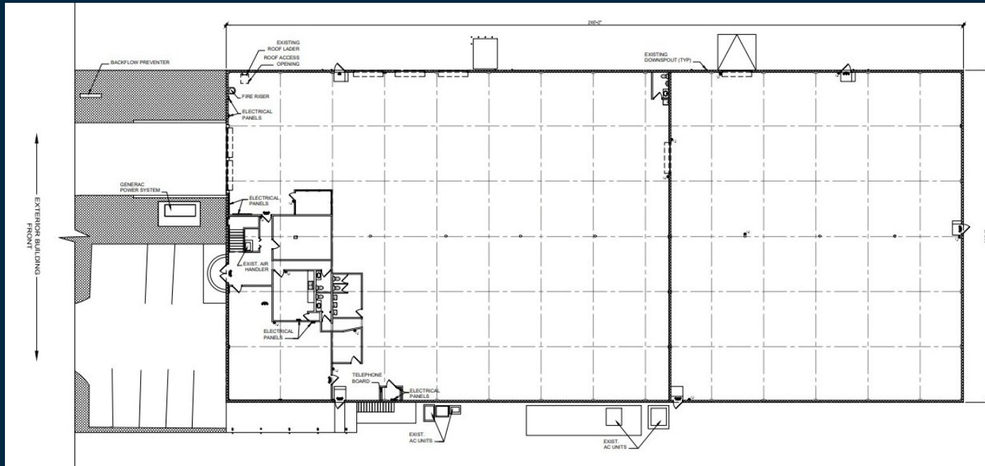
FIRST FLOOR
