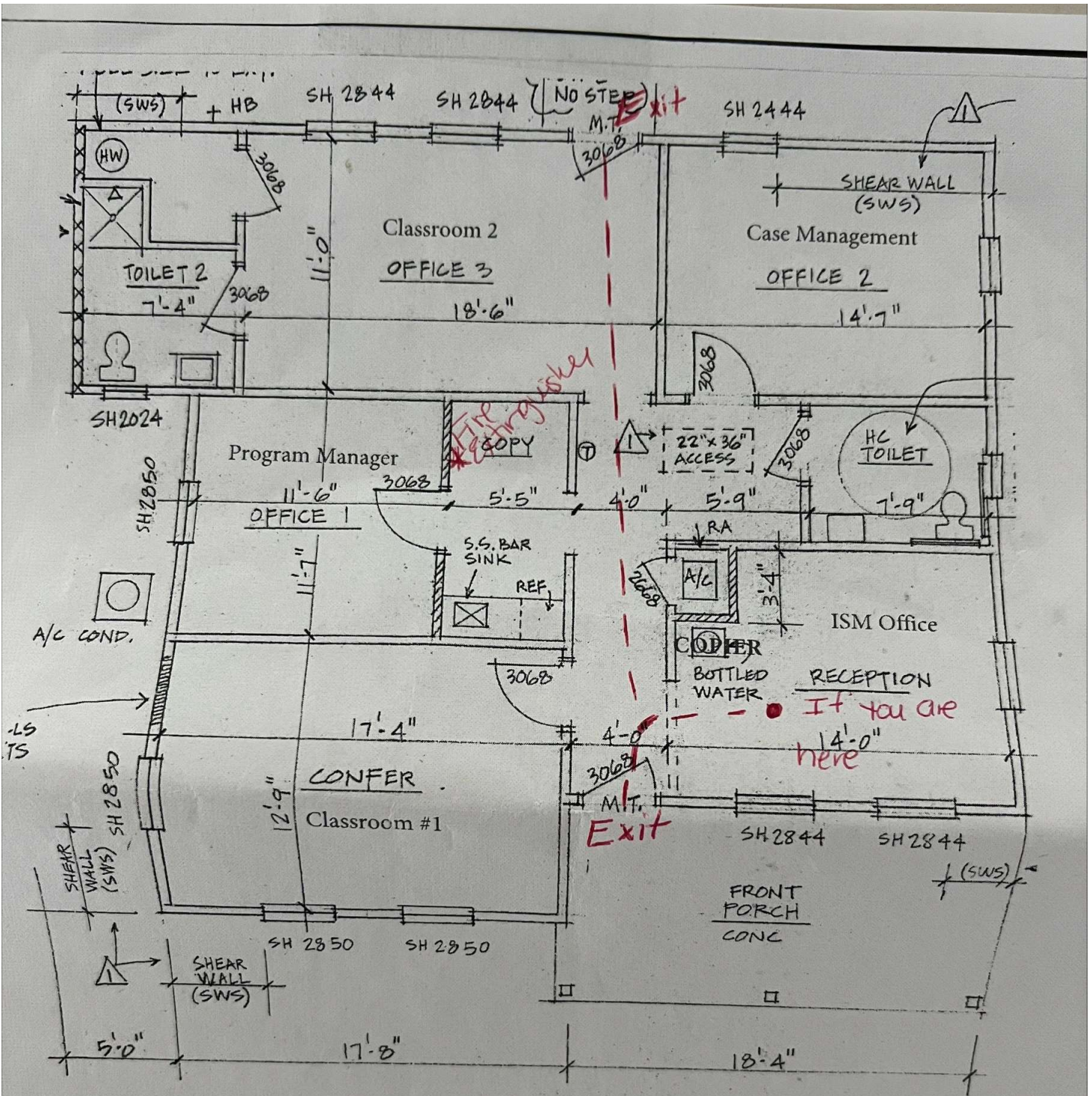
PROPOSED FLOOR PLAN 1/4" = 1'-0"
