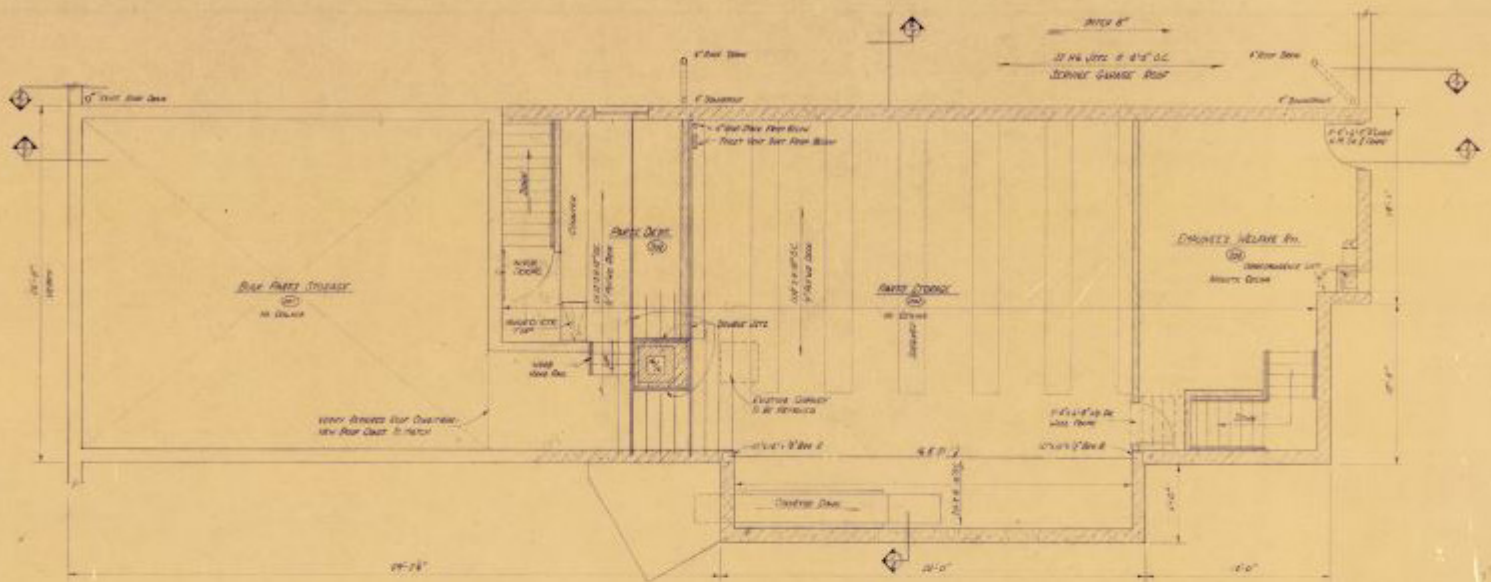
SECOND FLOOR PLAN & ROOF FINISHES DATE 8-1-14
