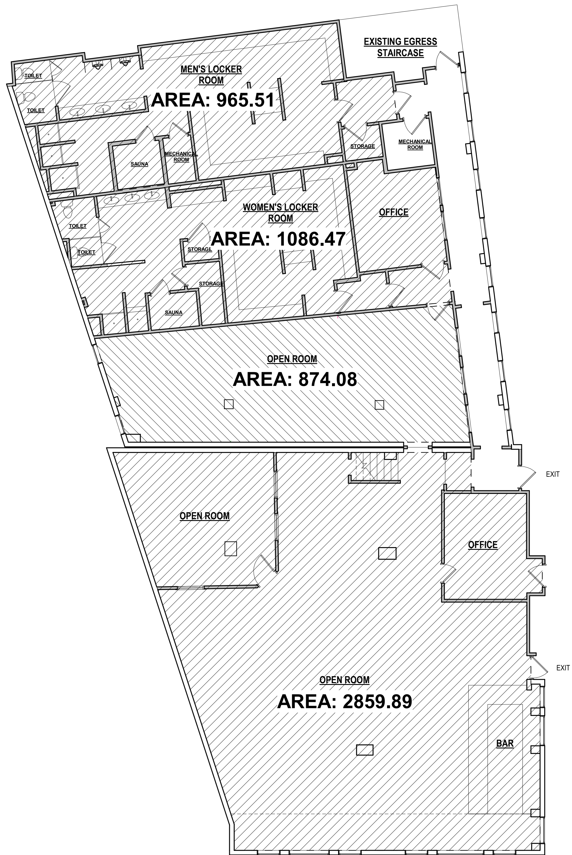
1 SECOND FLOOR - SQUARE FOOTAGES 1/8" = 1'-0"
