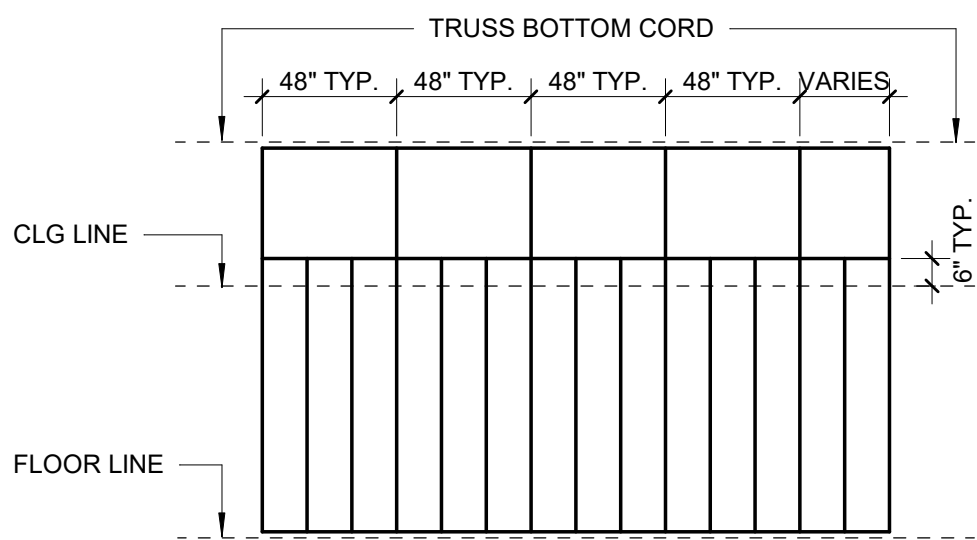
PARTITION "A" DIAGRAM
