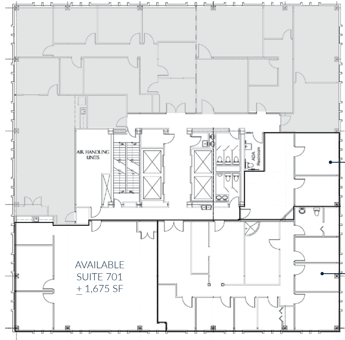
7TH FLOOR
