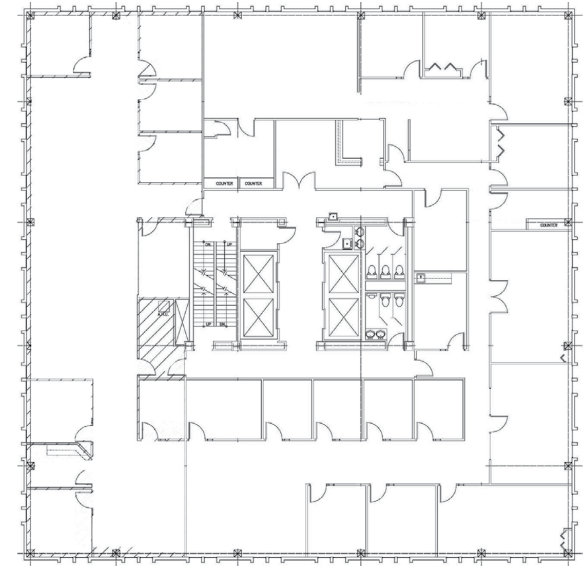
10TH FLOOR
