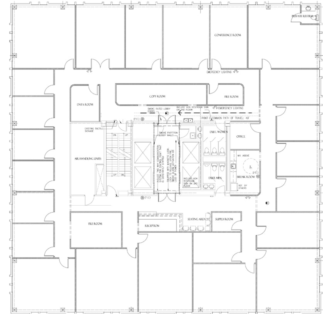
3RD FLOOR
