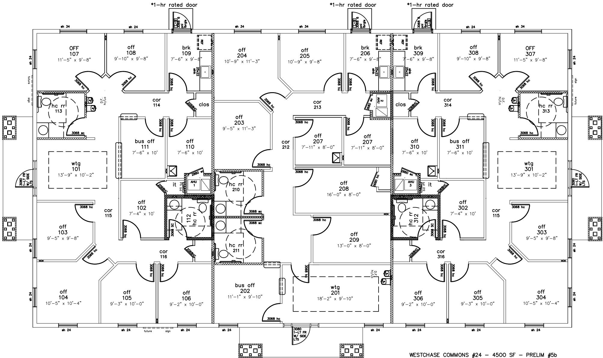
WESTCHASE COMMONS #24 - 4500 SF - PRELIM #5b WATERFORD CONSTRUCTION - 6.10.22 *preplumbs added
