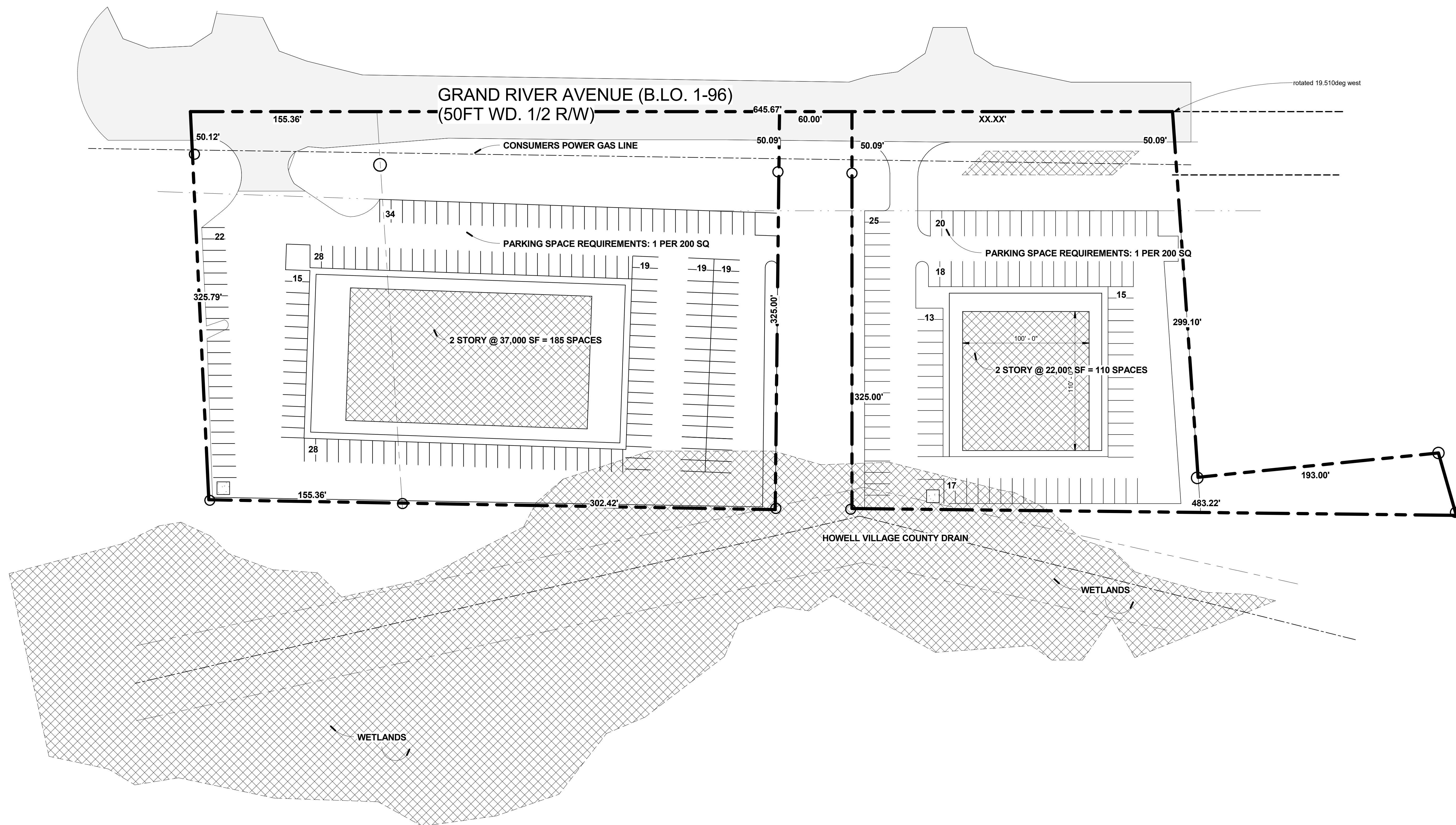
1 ARCHITECTUREAL SITE PLAN TWO STORY AS110 1" = 40'-0"
