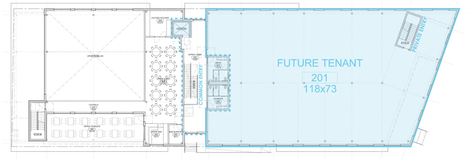
SECOND FLOOR PLAN 1/8" = 1'-0" 1
